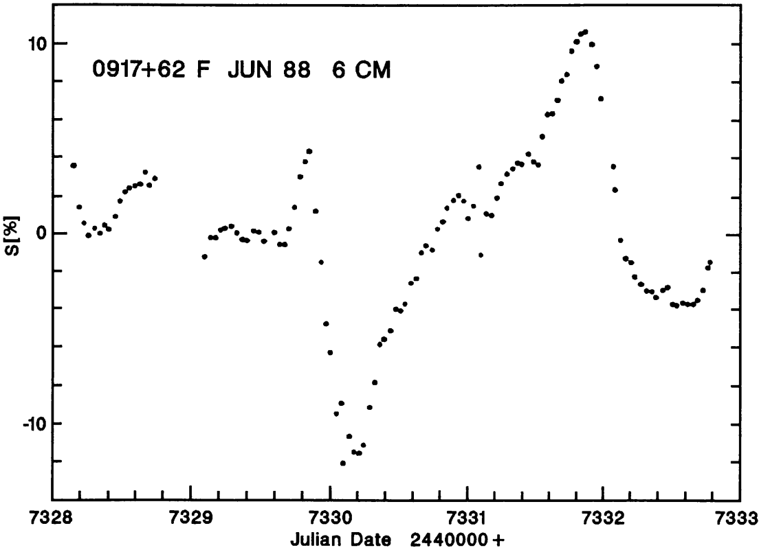
Figure 1. "Light curve" of the quasar 0917+624 at 6 cm wavelength, obtained with the Effelsberg 100 m radio telescope in June 1988. The y-axis gives the residual from the average flux density in per cent.
