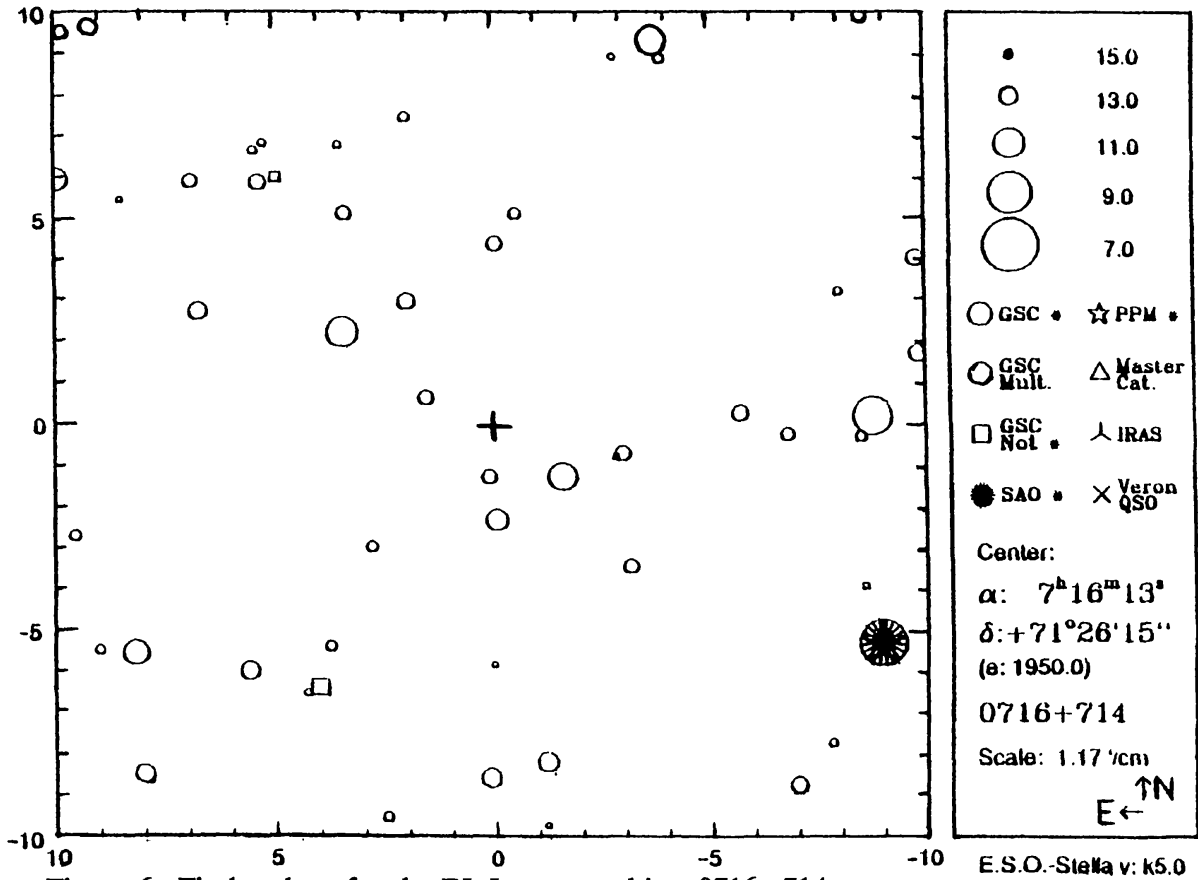
Figure 6. Finder chart for the BL Lacertae object 0716+714.
