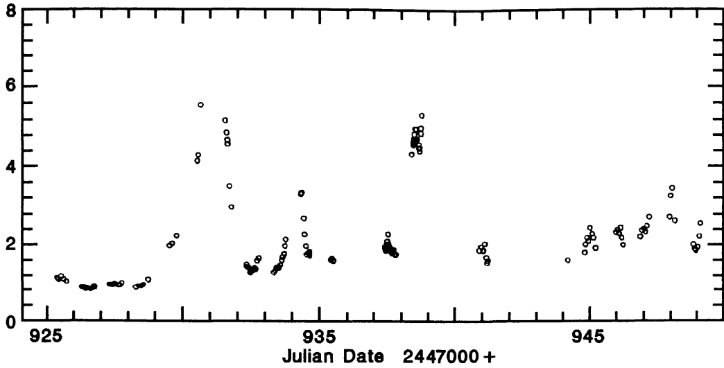
Figure 3. Light curve of the BL Lacertae object 0954+658 in the optical (R band). The y-axis gives brightness in arbitrary units, on a linear scale.
