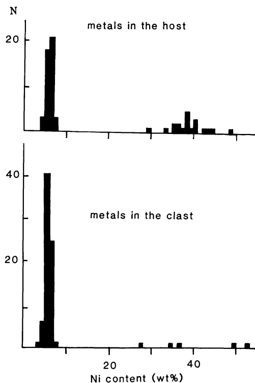
Fig. 5. The Ni content of grains of Fe-Ni metal in the host (upper) and those in the troilite-rich clast (lower).
