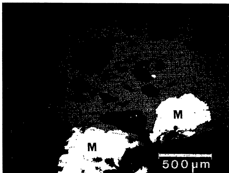
Fig. 2. Backscattered electron image of the part of the troilite-rich clast in Fig. 1. Black parts in the clast are chondrules and their fragments. M: metal, T: troilites.
