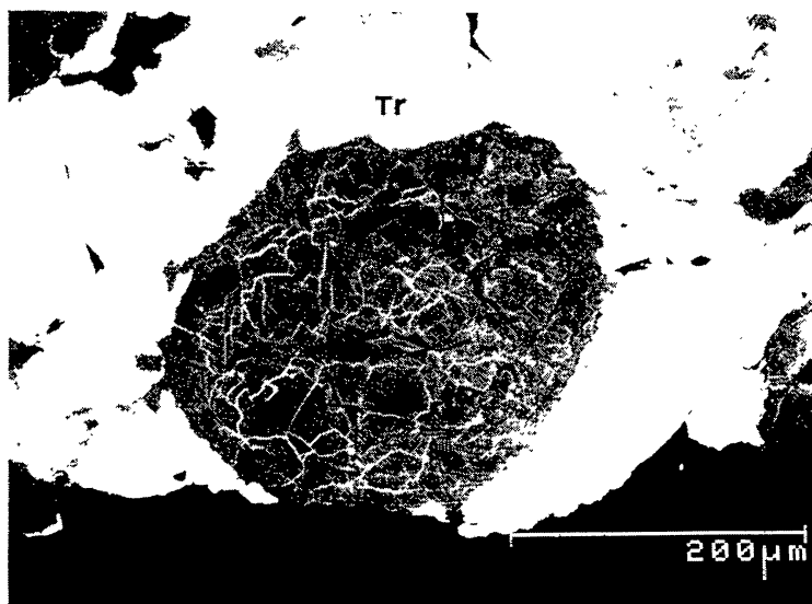
Fig. 10. Backscattered electron image of a chondrule enclosed in the troilite-rich clast. Olivines show compositional zoning. Ol: olivine, Tr: troilite.
