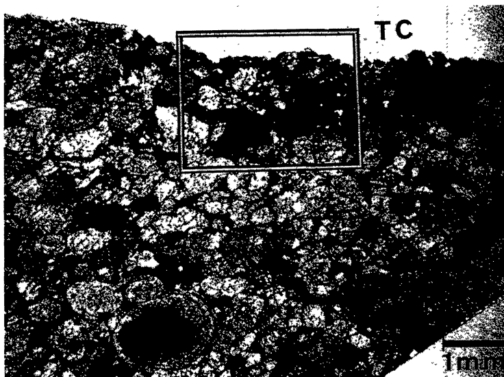
Fig. 1. Optical micrograph of thin section of the Moorabie chondrite. Chondrules have elongate morphology. Alignment of long axes of chondrules are observed along the horizontal axis. Regions in black are mostly opaque minerals. A troilite-rich clast (TC) is observed as the large region in black in the upper-right side of the figure. A part of the clast (within a square frame) is enlarged in Fig. 2.
