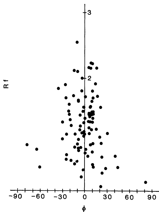
Fig. 3. R_f/\phi diagram of the elongate chondrule in a thin section of Moorabie (Fig. 1). The average direction of long axis of chondrules is fixed to be \phi=0 .
