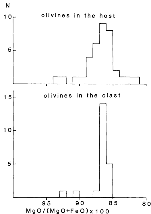
Fig. 4. Mg numbers ( MgO/(MgO+FeO) \times 100 ) of olivines in the host and those in the troilite-rich clast. Compositional ranges of olivines in the two regions coincide with each other.
