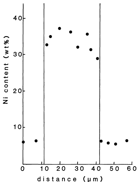
Fig. 6. Profile of Ni wt% (vertical axis) against distance (horizontal axis) in a metal grain in the host. Kamacite-taenite boundaries are shown as two vertical lines.
