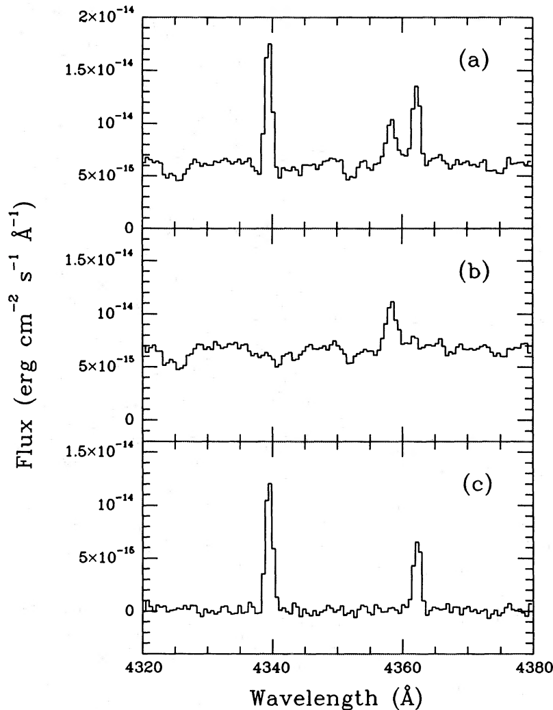
Figure 1. Spectra of the west knot of NGC 6543 taken with a 1200 \text{ l mm}^{-1} grating: (a) gross spectrum, (b) local sky spectrum in equivalent number of pixels and (c) sky subtracted spectrum. Note the accurate sky subtraction (including the Hg line at 4358 \text{ \AA} ) and the large strength of [O III] 4363 \text{ \AA} .
