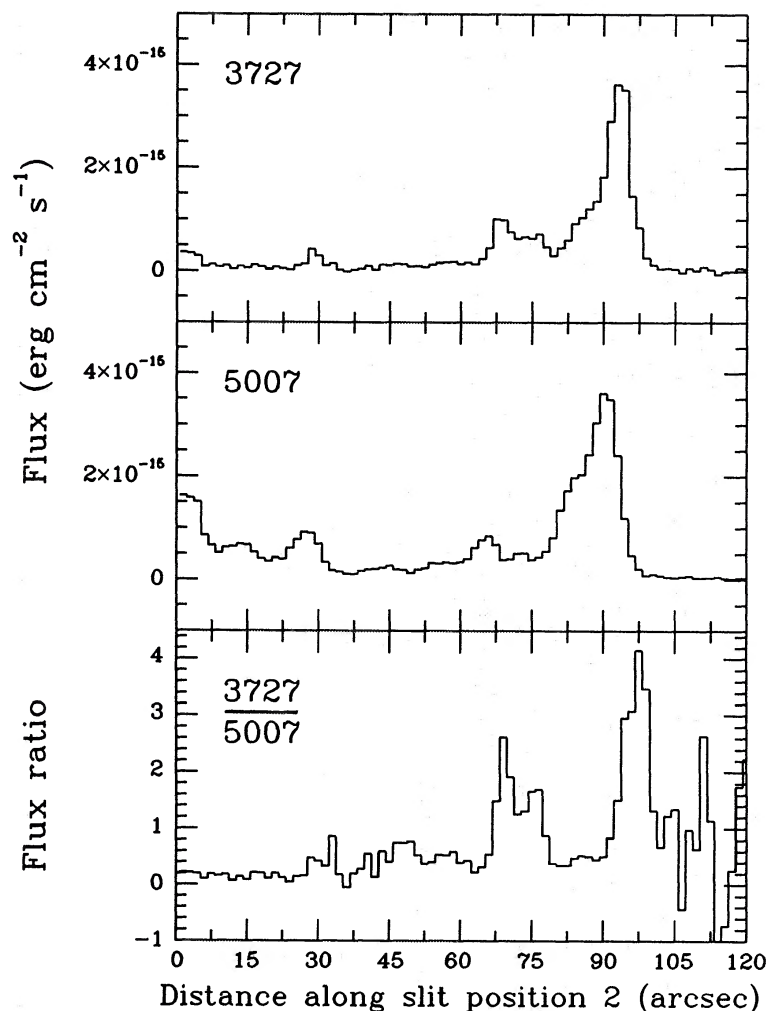
Figure 4. Spatial variation, along slit position 2 of [\text{O II}]\lambda 3727 , [\text{O III}]\lambda 5007 , and their ratio in NGC 6543. The sharp rise in the ratio at the edge of the halo is real and is not due to misregistration of the spectra or atmospheric dispersion effects. The nebular centre would be at -51 arcsec in this figure.
