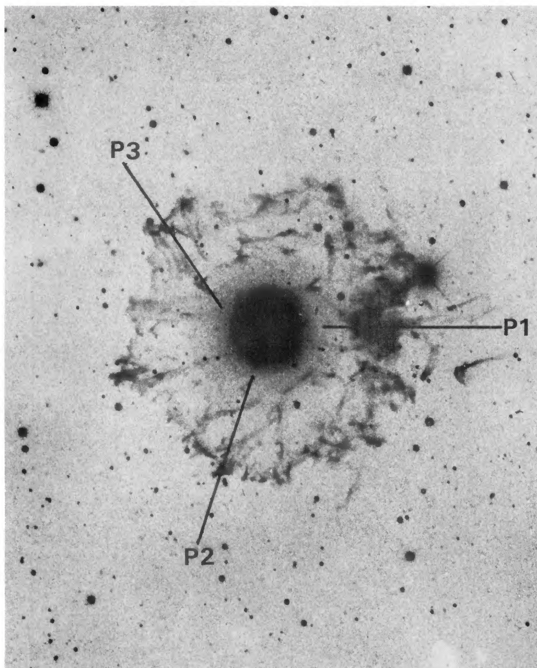
Plate 1. Deep exposure of the planetary nebula NGC 6543 showing details of the giant halo, with the inner nebula highly overexposed. North is at the top with east to the left. The slit positions marked are those at which we made observations. Note the filaments in the south-west outside the halo which are probably density enhancements in a large outer shell. This plate (by Millikan) has been contrast-enhanced by D. F. Malin.
