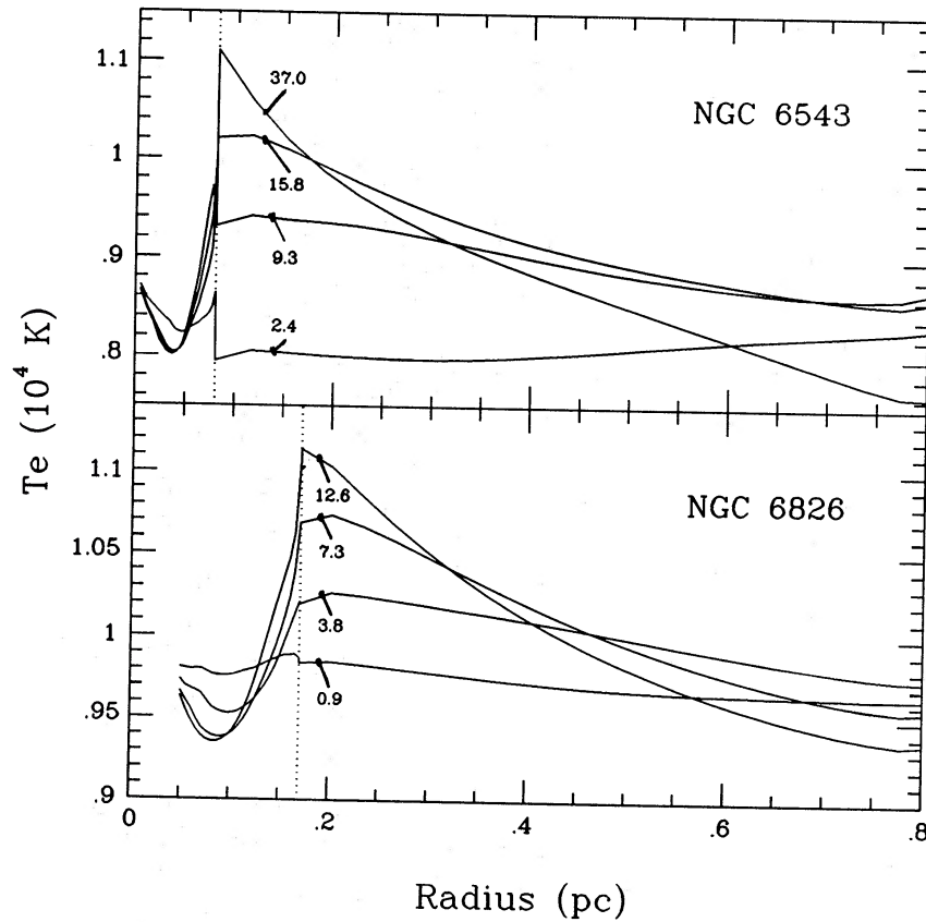
Figure 5. Variation of electron temperature with radius in various photo-ionization models of NGC 6543 and 6826. Each plot is labelled with \tau(H\text{ I}) for the entire model. The dotted line indicates the border between the core and the halo of the planetary nebula.
