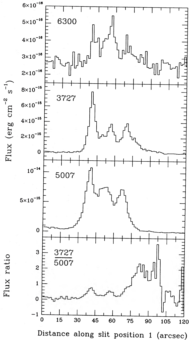
Figure 3. Spatial variation, along slit position 1 of [\text{O I}]\lambda 6300 , [\text{O II}]\lambda 3727 , [\text{O III}]\lambda 5007 , and the ratio of 3727/5007 in NGC 6543. The nebular centre would be at -55 arcsec in this figure.
