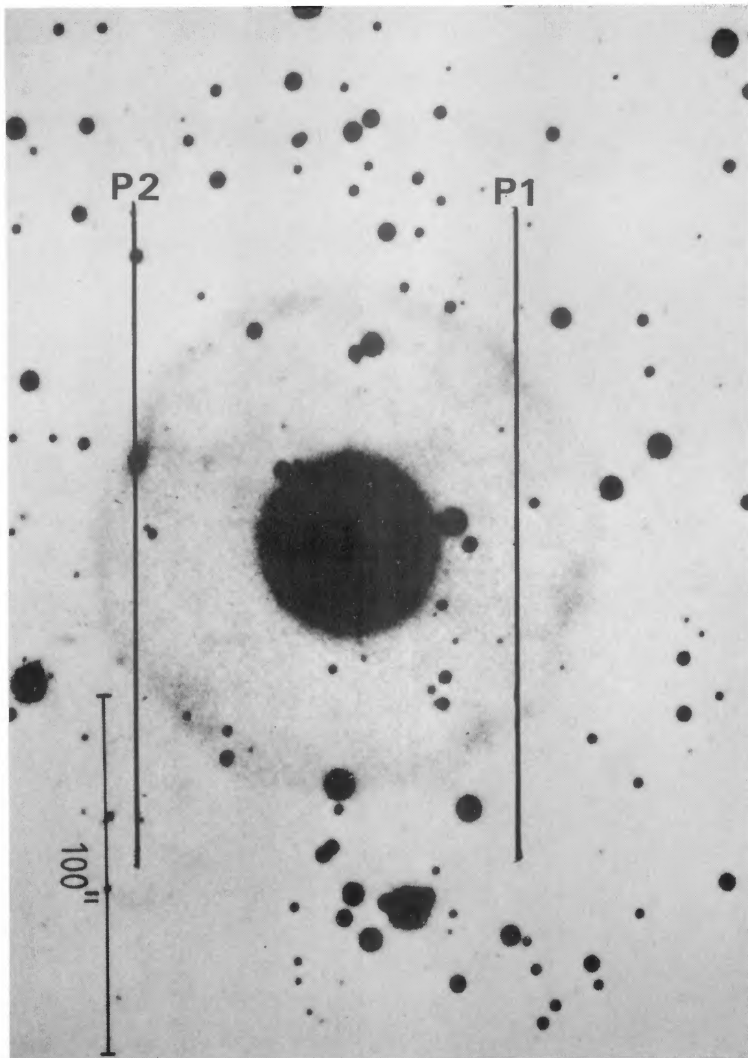
Plate 2. Deep exposure of the planetary nebula NGC 6826 showing its halo. The slit positions marked are those at which we made observations. The emission in the knot at the north edge of the halo on slit position 2 was found to be thermal.
