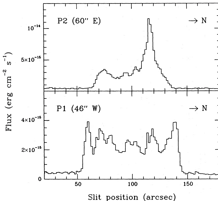
Figure 2. Spatial variation along the slit in the emission line [\text{O III}]\lambda 5007 for NGC 6826. Each slit position was oriented N-S and offset by the distance given in the plots (see Plate 2).
