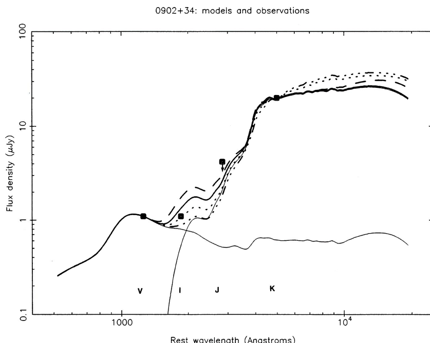
Figure 3: Comparison of the VIK fluxes of the radio galaxy 0902+34 (Lilly, 1988) with a model of two bursts: a recent 0.1 Gyr one plus an older one starting at different ages: 2 Gyr (dashed line), 3 Gyr (full line), 4 Gyr (dots), 5 Gyr (dashed-dots). The respective fluxes of the two bursts (0.1 Gyr and 3 Gyr) are also shown (thin lines), see text for details. The IMF is standard and the metallicity is half-solar. Normalization is at 4990 Å (K band in the rest frame).
