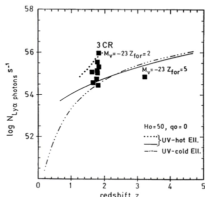
Figure 2: Number of Ly \alpha photons deduced from observations of Ly \alpha galaxies (Spinrad, 1988) compared to models for two redshifts of formation z_{\text{for}} = 2 and 5 (Rocca-Volmerange, 1988). Lyman continuum photons are absorbed by gas at a rate 70 %. Normalization is M_V = -23 .
