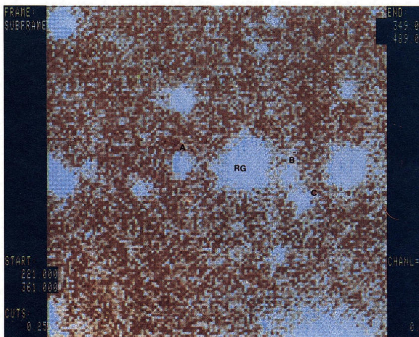
Figure 4: A 1-hour exposure in September 1987 towards a distant radio galaxy at a redshift z = 0.68 with the ESO 3.6-m telescope and a CCD detector through the R filter. The components have also been observed through the V, I filters.
