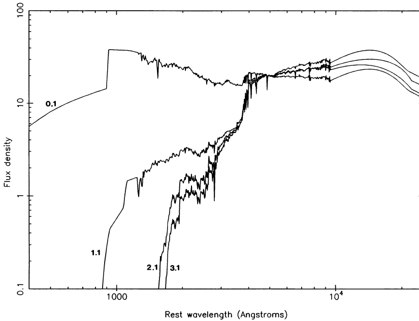
Figure 1: Synthetic spectra of a 1 Gyr burst at various ages indicated on each line in Gyr. Spectral resolution is 10 Å. Units are arbitrary. Normalization is at 4990 Å.
