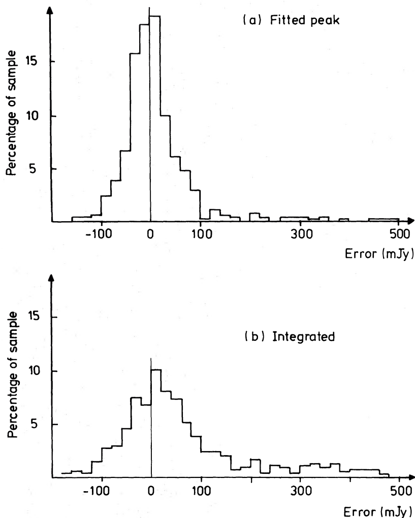
Figure 6. Typical histograms of the errors in measured flux densities of the Monte Carlo point sources when measured by (a) peak fitting, and (b) the integration algorithm.
