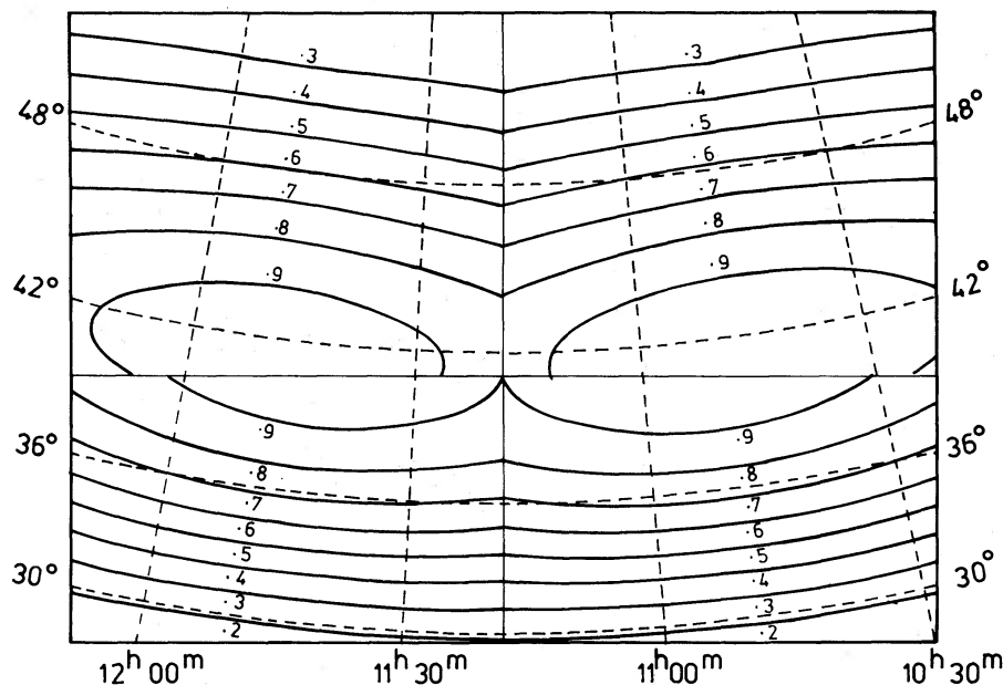
Figure 4. The effective attenuation pattern for a typical map consisting of four adjoining panels each synthesized from data appropriate to the right ascension of its own centre.
