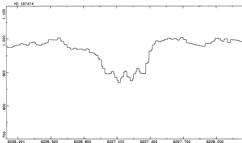
Figure 4: Resolved quadruplet observed in a CrII line.
