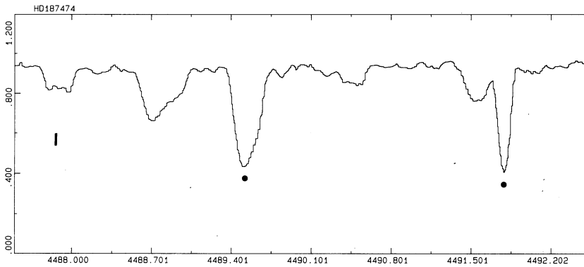
Figure 2: A portion of a Reticon spectrum of HD 187474. The points indicate two lines of FeII with different magnetic sensitivity. Note their different widths. The bar indicates a resolved Zeeman triplet in a CrII line.
