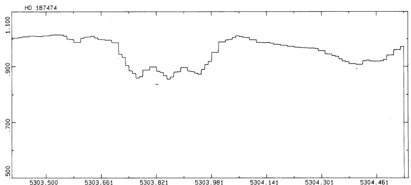
Figure 3: Resolved triplet observed in a FeII line.
