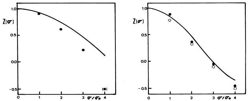
Figure 5: Zeeman broadening functions associated with different magnetic sensitive Fe I lines and the insensitive Fe I line ( \lambda 4491, z = 0.4 ). The full lines give the functions calculated with the parameters deduced from resolved Zeeman pattern ( B = 5 kgauss, A = 0.66 ). (a) The dots represent the observed broadening function associated with the sensitive magnetic line \lambda 4515 ( z = 1.03 ). (b) Observed broadening functions associated with the magnetic sensitive line \lambda 4520 (full dots) and \lambda 4489 (empty dots). The two lines have the same z value (1.5).
