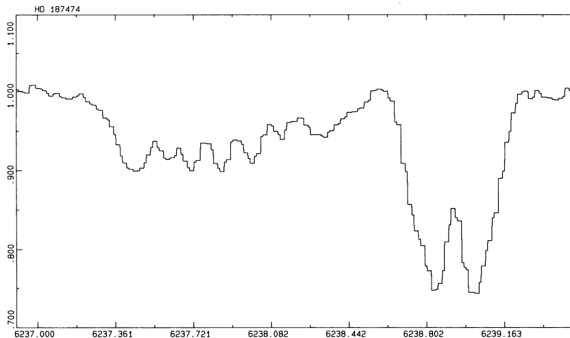
Figure 1: This spectral region of HD 187474 shows a doublet pattern in a FeII line and a very complicated structure due to simultaneous Zeeman splitting and blends of several lines.
