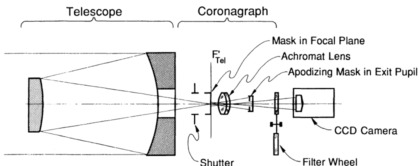
Figure 1: Optical configuration.
