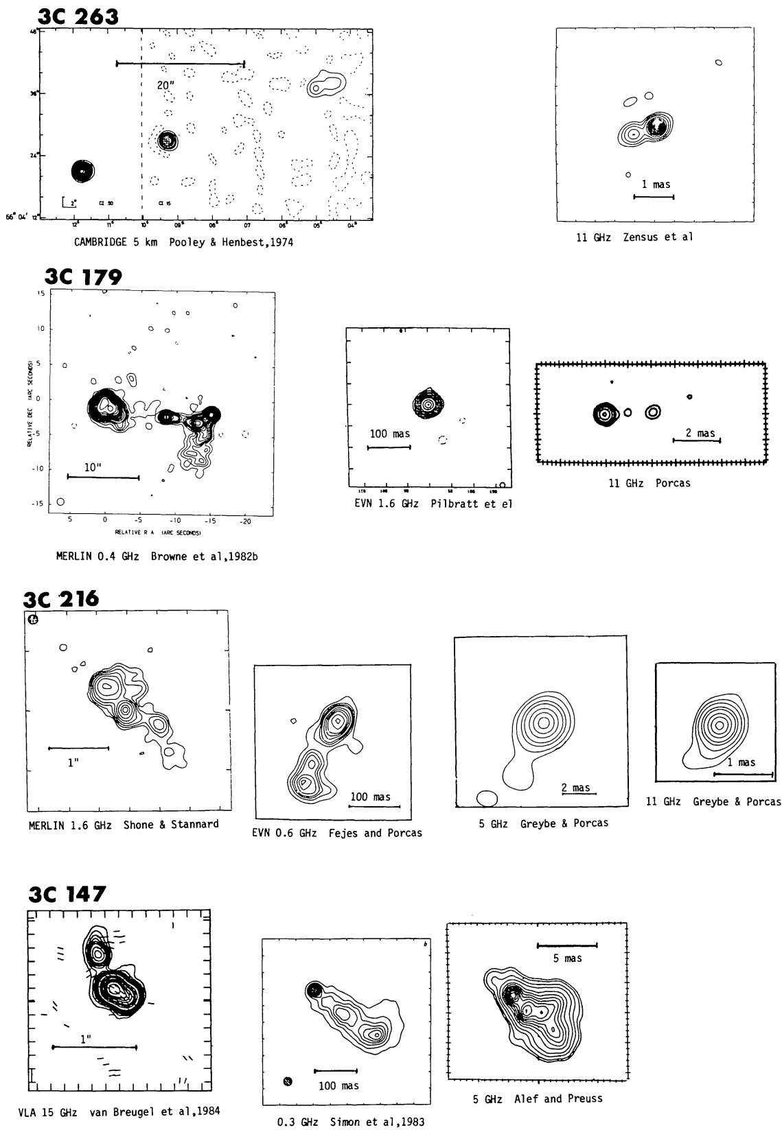
Figure 1: Arcsecond to mas structure of representative quasars.
