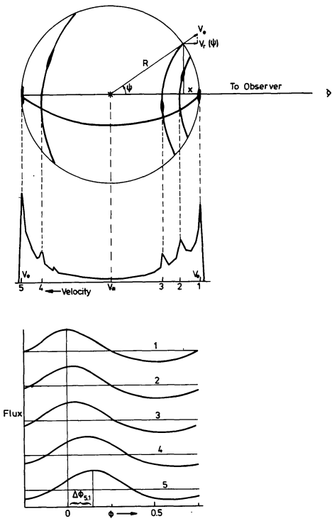
FIGURE 13. — Schematic representation of the uniformly expanding OH shell, the resulting single-dish spectrum, and the variations of different parts in the spectrum.
