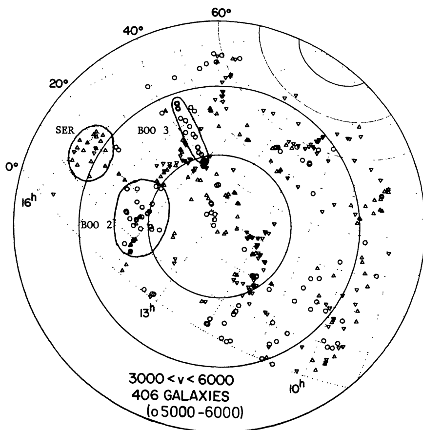
Figure 8 An equal-area plot in galactic coordinates of galaxies brighter than m_B = 14.5 above b = +40^\circ . The galactic pole is at the center, the circles are at b = 30^\circ, 50^\circ , and 70^\circ . Right ascensions and declinations are indicated by dotted curves. Galaxies whose absolute magnitudes are fainter than -20.0 (on the H_0 = 50 distance scale) have been omitted. The various symbols denote the following velocity bins: \nabla ( 3000\text{--}4000 ), \triangle ( 4000\text{--}5000 ), \circ ( 5000\text{--}6000 \text{ km s}^{-1} ). Reproduced by courtesy of M. Davis (except for the contours).
