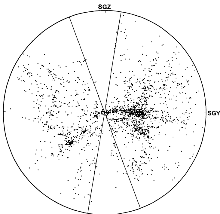
Figure 3 All 2175 galaxies in the Nearby Galaxy Catalog (NGB) projected onto the SGY - SGZ plane. The SGY -axis is directed toward supergalactic longitude 90^\circ , supergalactic latitude 0^\circ ( \ell^{\text{II}} = 227^\circ , b^{\text{II}} = +83^\circ.7 ), the SGZ -axis toward supergalactic latitude 90^\circ ( \ell^{\text{II}} = 47^\circ.4 , b^{\text{II}} = +6^\circ.3 ). The radius of the outer boundary is 60 Mpc. The galactic zone of avoidance ( b < 15^\circ ) is contained within the opposed wedges tilted by 6^\circ with respect to the SGZ -axis. There is a zone of incompleteness ( \delta < -45^\circ ), which is projected across most of the southern supergalactic hemisphere. Figures 3–6 are reproduced by courtesy of R. B. Tully (92).
