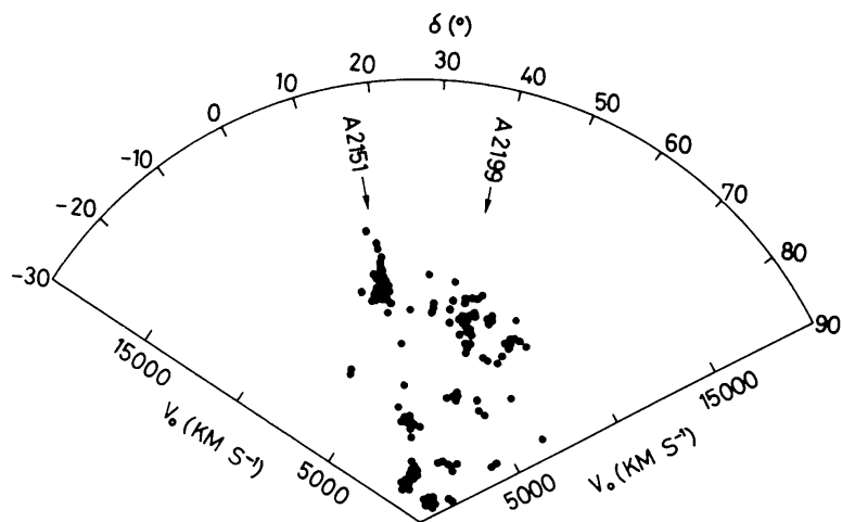
Figure 19 The Hercules supercluster. “Cone diagram” of velocity versus declination for galaxies between 15 h 30 m and 17 h 0 m right ascension. Reprinted by courtesy of Tarenghi et al. (88) and the Astrophysical Journal .
