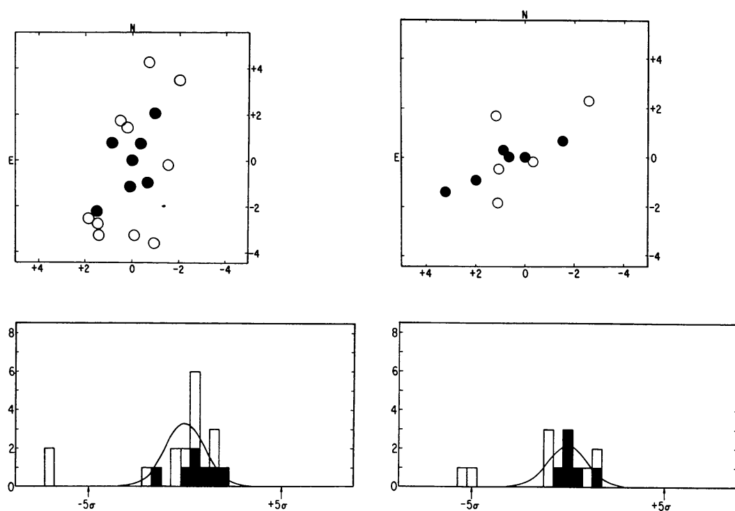
Figure 22 Sky (top) and velocity distribution (bottom) of two second-order clusters. Solid circles and rectangles are rich clusters, open circles and rectangles are groups and poor clusters. Bins in bottom figures have width of the velocity dispersion \sigma . Nonmember galaxies closest in velocity to that of the supercluster are also shown. Reproduced by courtesy of Ford et al. (35) and the Astrophysical Journal .
