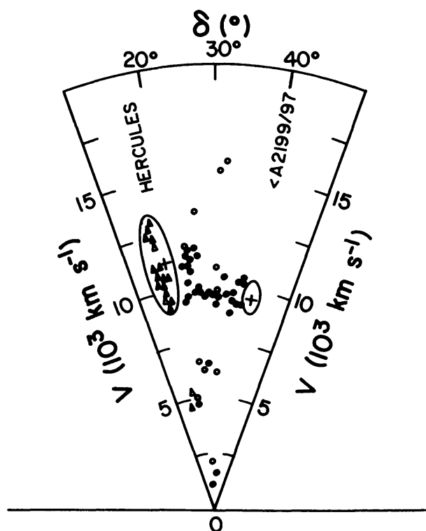
Figure 17 The Hercules supercluster. Radial velocities of galaxies between the two principal groups of clusters (which have been indicated by elliptical contours) plotted against declination. Data for Hercules (triangles) are from Tarenghi et al. (88, 89); the ellipse for A 2199/A 2197 is from Thompson & Gregory (90). Reproduced by kind permission of Chincarini et al. (15) and the Astrophysical Journal .
