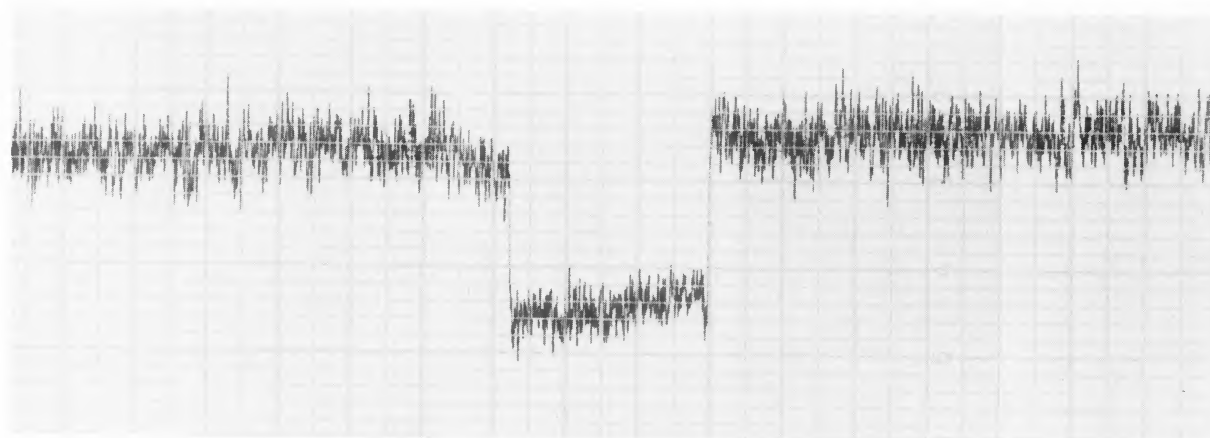
FIG. 2. The light curve of the 7 October 1981 occultation of SAO 187124 by 88 Thisbe observed near Otter Creek Reservoir in central Utah.
