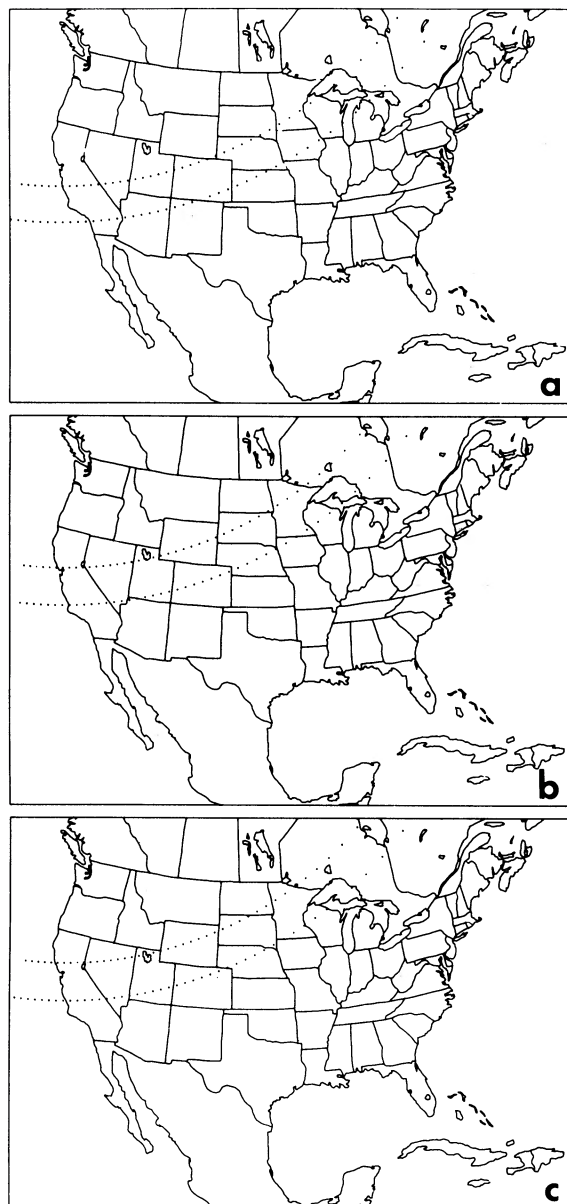
FIG. 1. The predicted ground track of the 7 October 1981 occultation of SAO 187124 by 88 Thisbe based on (a) plates taken at Lick Observatory on 27 September 1981, (b) a plate taken at Lick on 4 October 1981, and (c) plates taken at the Flagstaff Station of the U.S. Naval Observatory on 6 October 1981.
