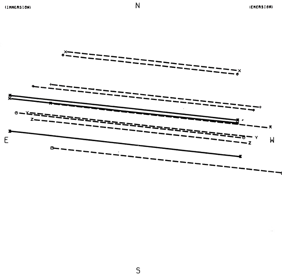
FIG. 3. Chords across Thisbe, uncorrected for the response times of visual observers. Solid lines represent photoelectric observations; dashed lines are chords derived from visual observations. Table I lists the observing sites corresponding to the chords, beginning with the northernmost chord.
