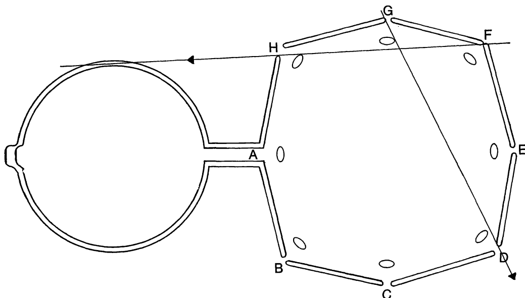
FIG. 8. A sketch shows two of the “missing” lunar alignments which are unmarked by the sides of the Octagon. If these alignments were deliberate, they would account for the narrowness of the gap at F , the relatively short length of wall HA , and the positions and sizes of mounds H and G .
