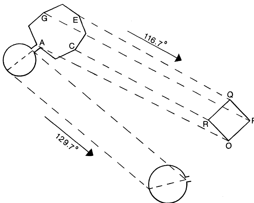
FIG. 5. A sketch shows the parallel-displaced relationships between the Fairground and Observatory Circles and between the Square and the Octagon. The azimuths of the displacements mark southern extreme lunar rising points.
