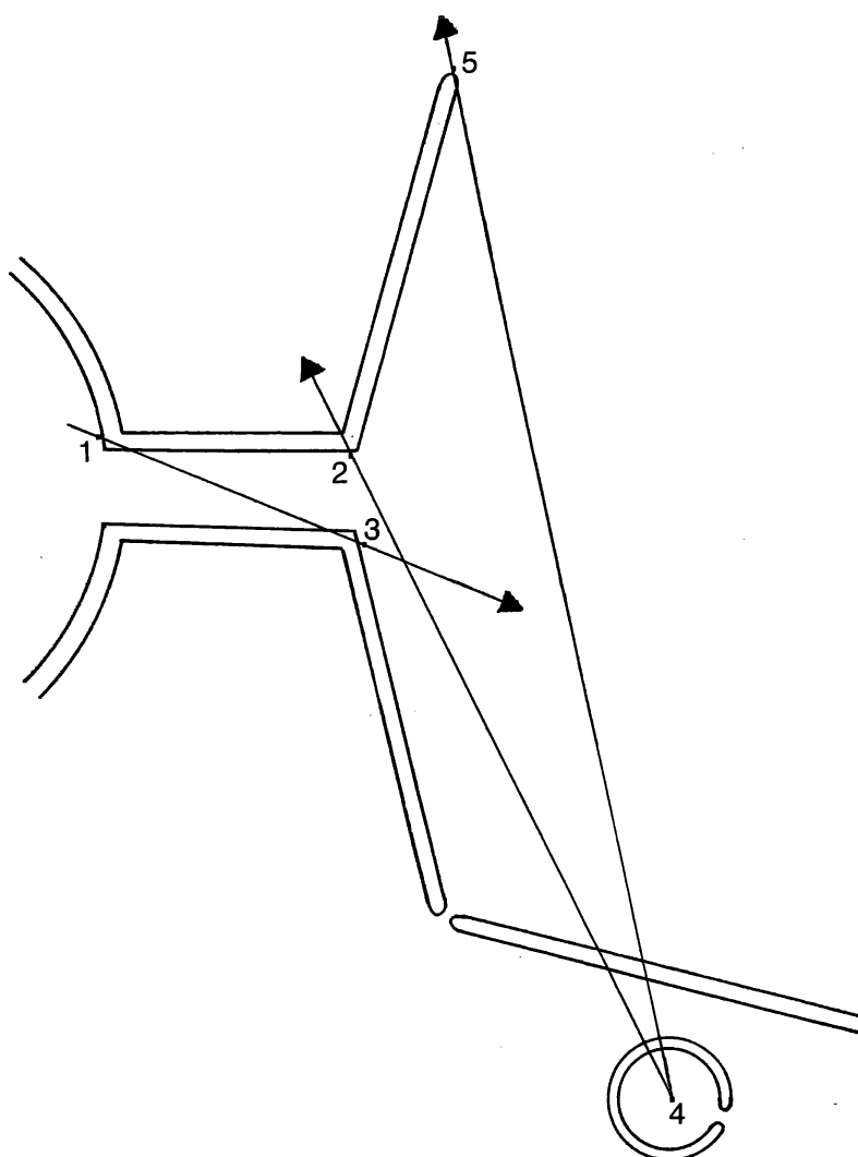
FIG. 7. The arrows in this plan show lunar alignments diagonally across the avenue (1–3) and across the ends of wall HA as seen from the centre of the small circle (4–2 and 4–5).
