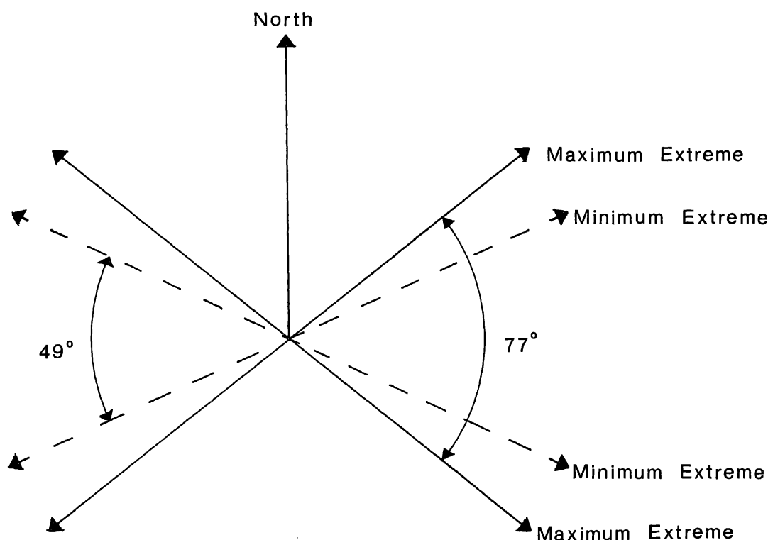
FIG. 6. The extreme azimuths of the lunar rise-set points at Newark are shown by the arrows. The azimuths shown are approximate in that the effects of horizon altitude and refraction have been ignored. When the Moon is at a position for maximum extremes, the extreme north and south moonrises in a given month are separated by 77^\circ ; at the position for minimum extremes, the extreme moonrises are separated by 49^\circ .
