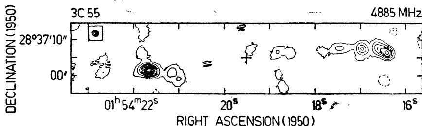
Figure 2. 3C 55: peak flux is 174 mJy.
