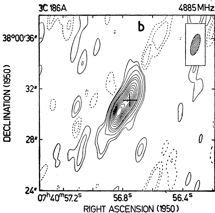
Figure 3. 3C 186: peak flux is 128 mJy. The optical position is from Argue and Kenworthy (1972).
