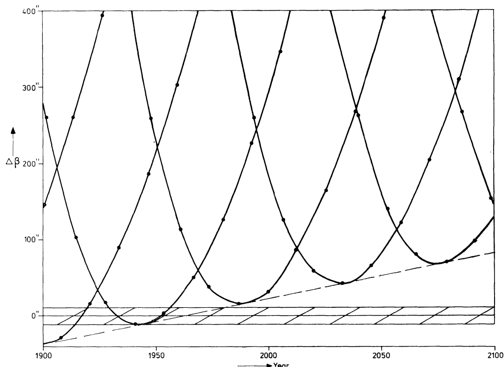
FIGURE 1. Plot of all close (less than 400'' ) Mercury- \epsilon Gem conjunctions. \Delta\beta is the latitude of the star minus the latitude of the planet. The solid lines connect conjunctions with 13 years' interval; the dashed line touching these parabolas represents the most northern position of the planet which can be reached. The band around \Delta\beta = 0 indicates the area where occultations take place, as for instance in 1940 and 1953. Due to the secular changes in the planetary orbit and the proper motion of the star, from 1980 no occultation is possible, as can be seen from the figure. The plot is for the period 1900 to 2000.
