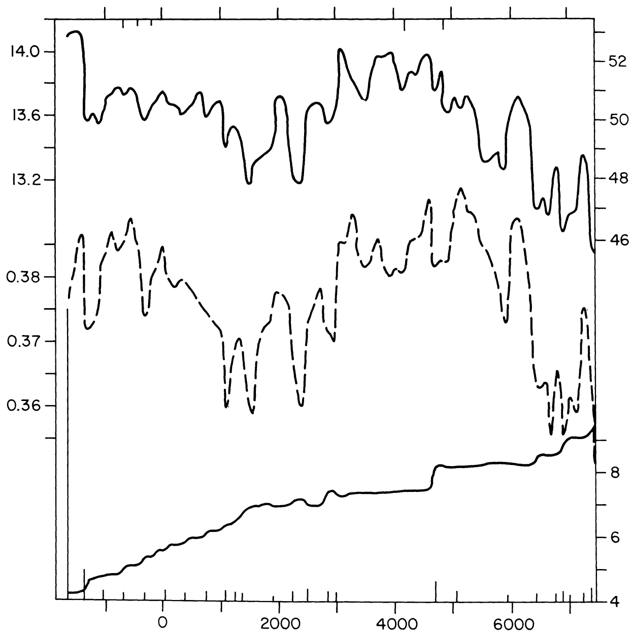
Figure 1. The variations in the orbital elements a (and P ), e and i between the encounter with Saturn in -1664 and about the year 7400. The vertical lines inside the frame of the figure represent close approaches to Saturn (bottom) and Uranus (top). Only approaches \Delta within 2 AU are marked, the lengths of the lines being proportional to \Delta^{-1} - 0.5 .
