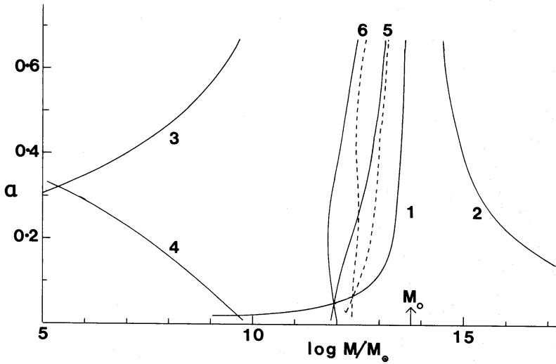
Figure 2. Various characteristic masses are here plotted, as a function of \alpha (equation (2.1)), for the case when \Omega = 0.2 , h = 0.5 and F_f (the fraction of cosmic matter still in gaseous form) is 0.1. The amplitude of (2.1) is normalized by choosing the scale mass M_0 to have the value (2.19). The curves are as follows: (1) The typical mass for which t_{\text{dyn}} = t_0 (i.e. t_{\text{turn}} = t_0/2 ). (2) The mass M_{1 \text{ per cent}} such that 1 per cent of the material is in units with t_{\text{dyn}} < t_0 . (3) The typical mass for which t_{\text{dyn}} = t_{\text{rec}} . (4) The typical mass for which T_{\text{virial}} = 10^4 K. This sets the minimum halo mass within which gas can condense if H and He are the dominant cooling agents. (5) The typical mass for which t_{\text{cool}} = t_0 . The luminous cores of galaxies will have a characteristic maximum mass 0.1 f times this value (see Table 1). (6) The typical mass for which t_{\text{cool}} = t_{\text{dyn}} . The continuous curves 5 and 6 correspond to cooling by H and He alone, and the dashed curves to the inclusion of heavy elements with 10 per cent of their 'cosmic' abundance.
