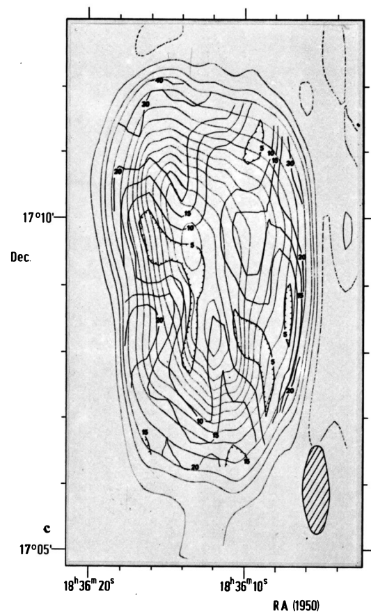
Fig. 8. Maps of 3C 386 made at 21 cm. a The total intensity shown with contours of -5 (dashed), 5, 15, 25, 50, 100, 150, 200, 250, 300, 350, 400, 450, 500 and 550 mJy/beam. b The linearly polarized intensity and position angle shown with contours of 5, 15, 25, 37.5, 50, 62.5, 75 and 100 mJy/beam. c Contours showing the percentage of linear polarization superimposed on a total intensity map
