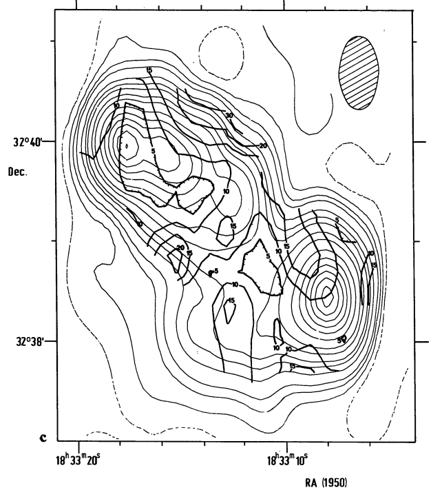
Fig. 2. Maps of 3C 382 made at 21 cm. a Contours showing the total intensity distribution with values of -5 (dashed), 5, 15, 25, 50, 75, 100, 150, 200, 300, 400, 500, 600, 700 and 800 mJy/beam. b Contours of linearly polarized intensity and lines showing the position angle distribution. Contour values are, 5, 15, 25, 37.5, 50, 67.5, and 75 mJy/beam. c Contours of the degree of linear polarization superimposed on total intensity contours
