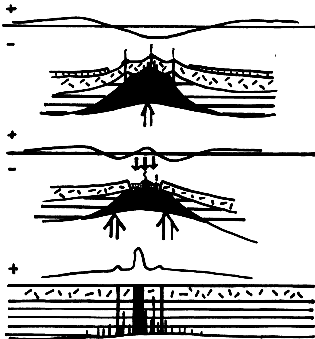
Figure 3 Structure and Bouguer anomalies at swell, active, and failed rift structures. Bouguer anomaly over a swell (top) is negative and attributable to mass deficient, partly melted asthenosphere (black) rising (open arrow) through the lithospheric mantle (lined) and doming continental crust (dashes). Volcanoes crest the dome and overlying sediments (dots) form a bordering scarp (based on the Ahaggar). A central positive Bouguer anomaly is related to axial dikes in an active rift (middle figure). A broad negative anomaly is attributed to the persistent asthenosphere swell (black, open arrows). The greater mass of the axial dike system due to mafic and ultramafic rocks makes the rift sink (solid arrows) (based on Kenya Rift). In an inactive rift (bottom) with no sediments the axial dikes are exposed cutting the continental crust but are more abundant in the lithospheric mantle. A sharp positive Bouguer anomaly marks the axial dike (based on the Great Dike of Rhodesia).
