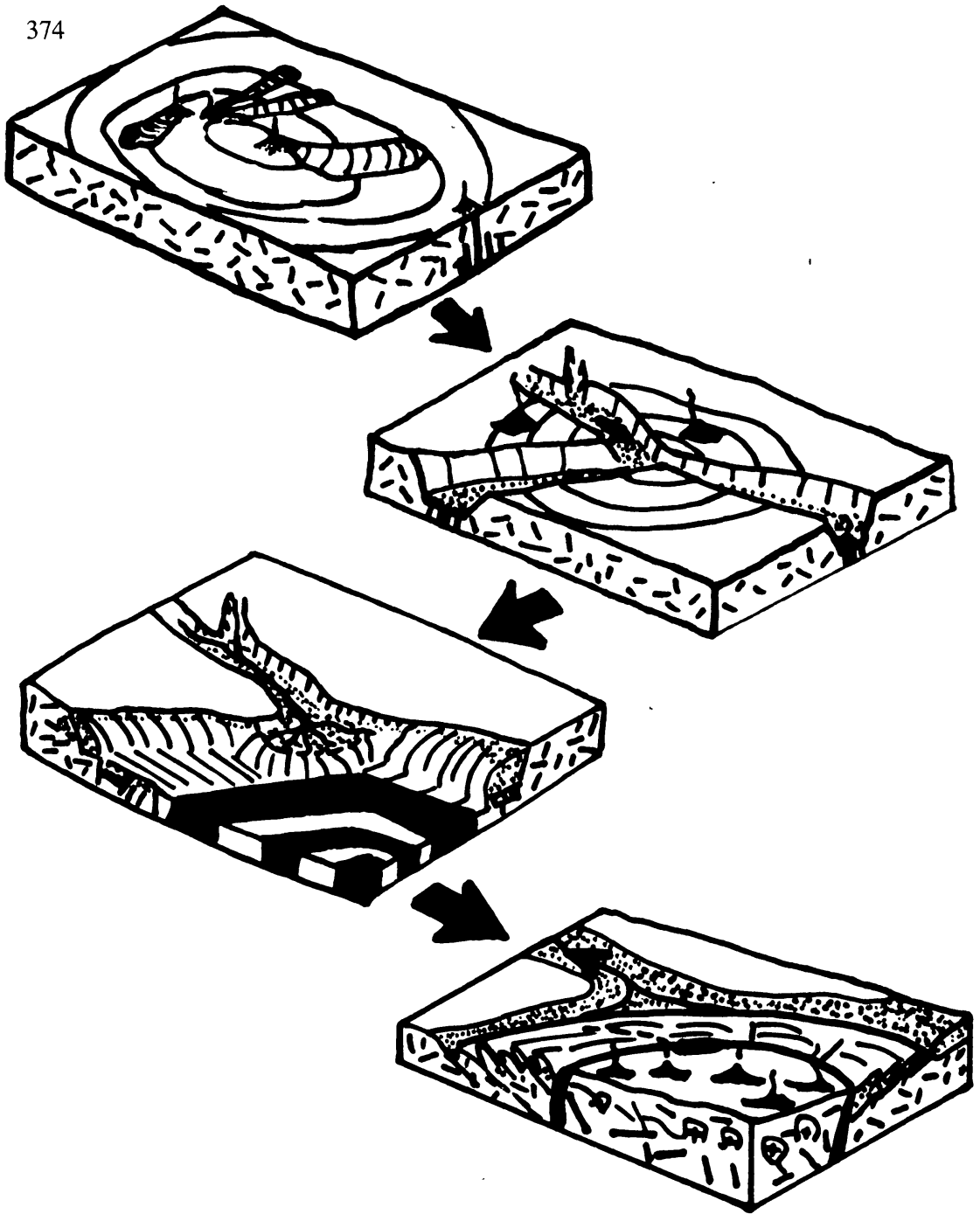
Figure 1 The sequence of swell, rift, continental rupture, and collision in aulacogen formation. A swell within a continent (top left) is crested with volcanoes from which lavas flow and evolves into a three-rift system (upper right) with volcanoes, sediment fill (stippled), and axial dikes. Two of the rifts develop to a continental margin (lower left) and ocean (striped) forms on their sites. A miogeoclinal wedge (stippled) is deposited along the new continental margin and a delta progrades down the failed rift to lie on ocean floor. Later (bottom right) another continent crosses the closing ocean and two continents collide. Rocks of the miogeoclinal wedge are thrust onto the continents and eroded by a river flowing down the aulacogen in the reversed direction. A suture zone (vertical black lines) marks the former site of the ocean and igneous rocks develop in the thickened continent on one side.
