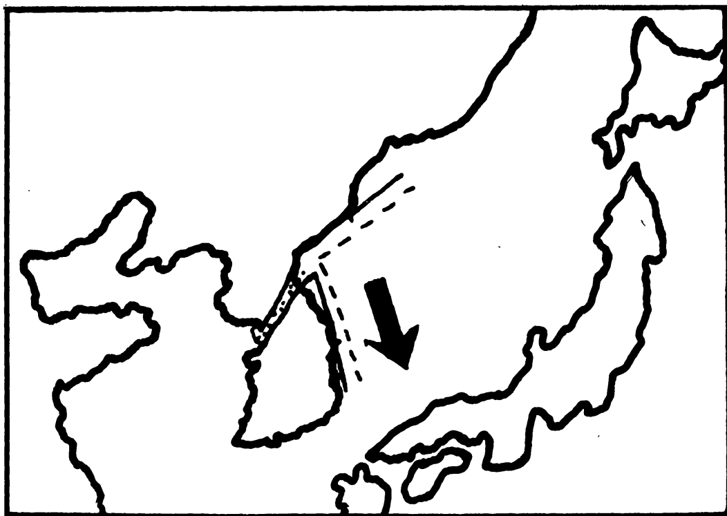
Figure 4 The Neogene and Recent Seoul-Wonsan graben (stippled) may be a failed rift associated with the opening of the Japan Sea.
