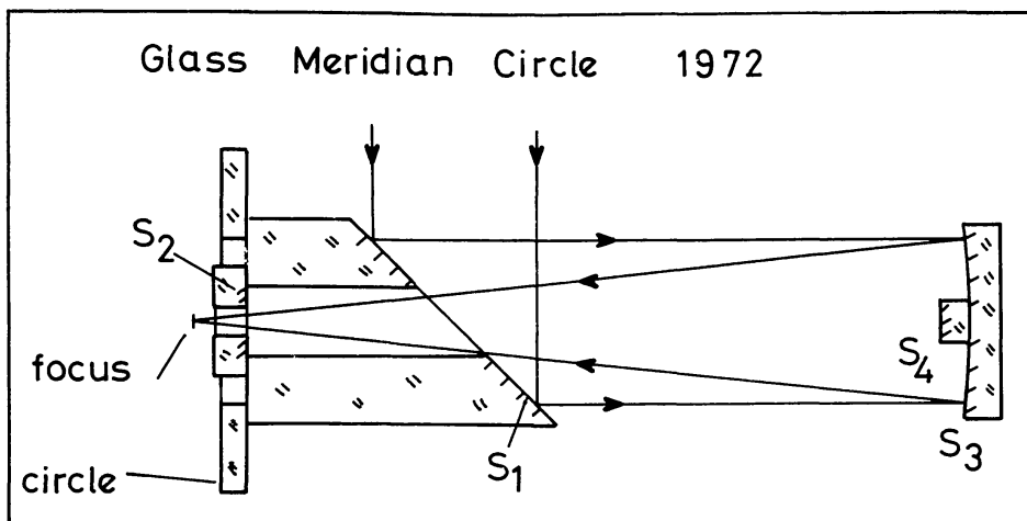
Fig. 3. The Glass Meridian Circle in the new version where the fixed telescope and the autocollimator have been combined in the mirror S_3 . The mirror S_4 is cemented to S_3 and since its center of curvature coincides with the focus of S_3 , it can serve to control the tilt of S_3 .
