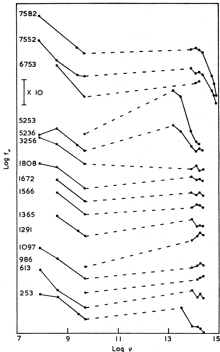
FIG. 7. The spectra of 15 galaxies for which both radio and infra-red measures exist. The magnitudes were converted to fluxes according to the calibration of Becklin, quoted by Glass & Feast (1973b, in preparation). The sources of the data outside the JHKL region are given in the text.
