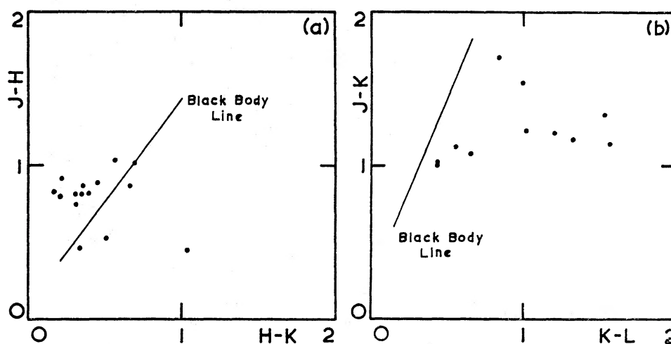
FIG. 5. Colour-colour diagrams of galaxies. (a) shows a clumping around J-H = 0.8 , H-K = 0.2 characteristic of late-type giants. The diagram (b) shows the L -excesses which move the colours away from the blackbody line.
