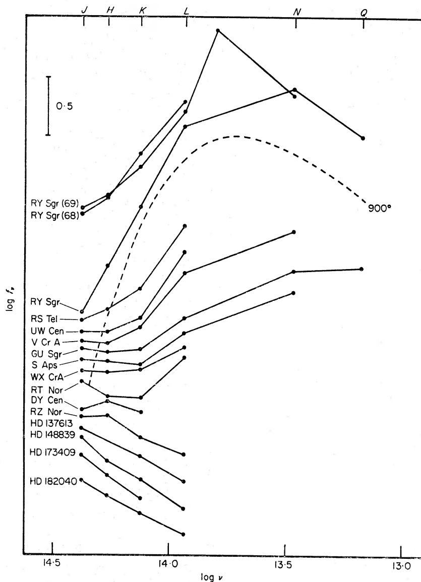
FIG. 2. \log F_v - \log v diagram for RCB and HdC stars. Ordinate arbitrary except that the observations of RY Sgr in 1968, 1969 and 1972 are correctly placed relative to one another. A 900^\circ black body is shown for comparison.
