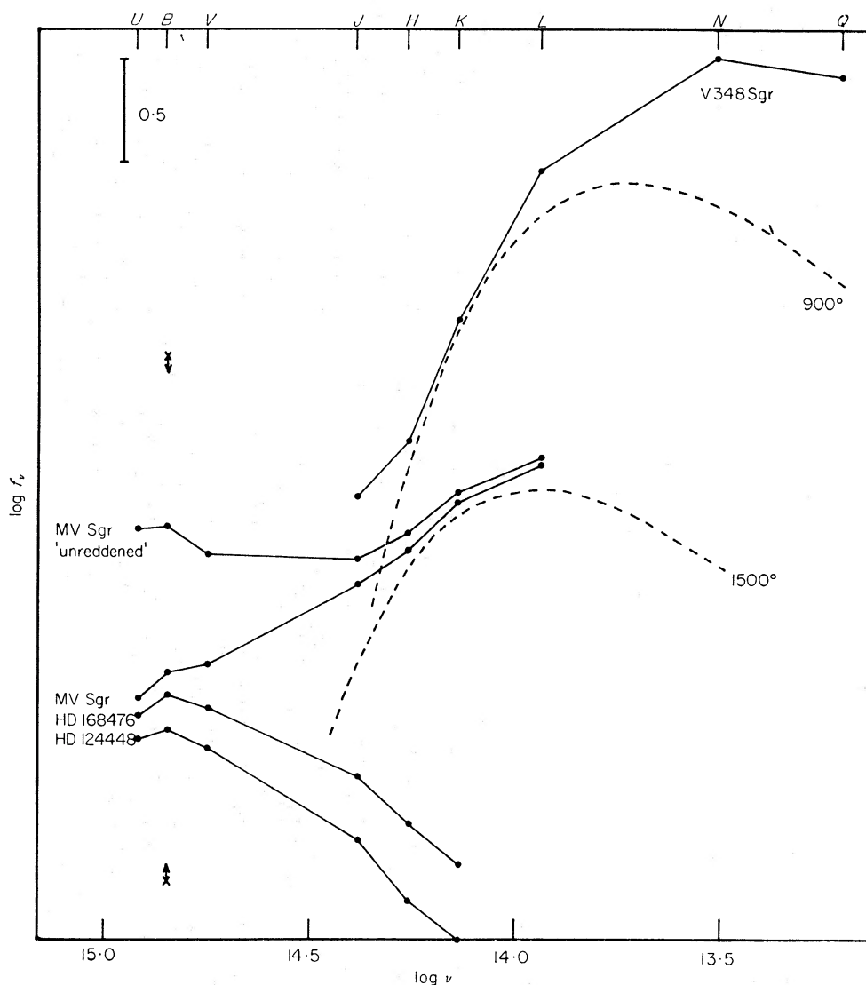
FIG. 3. \log F_\nu - \log \nu plot for helium stars, MV Sgr and V348 Sgr. The crosses indicate the approximate B flux of V348 Sgr at maximum and at minimum. Black-body fluxes at 900° and 1500° are shown for comparison.
