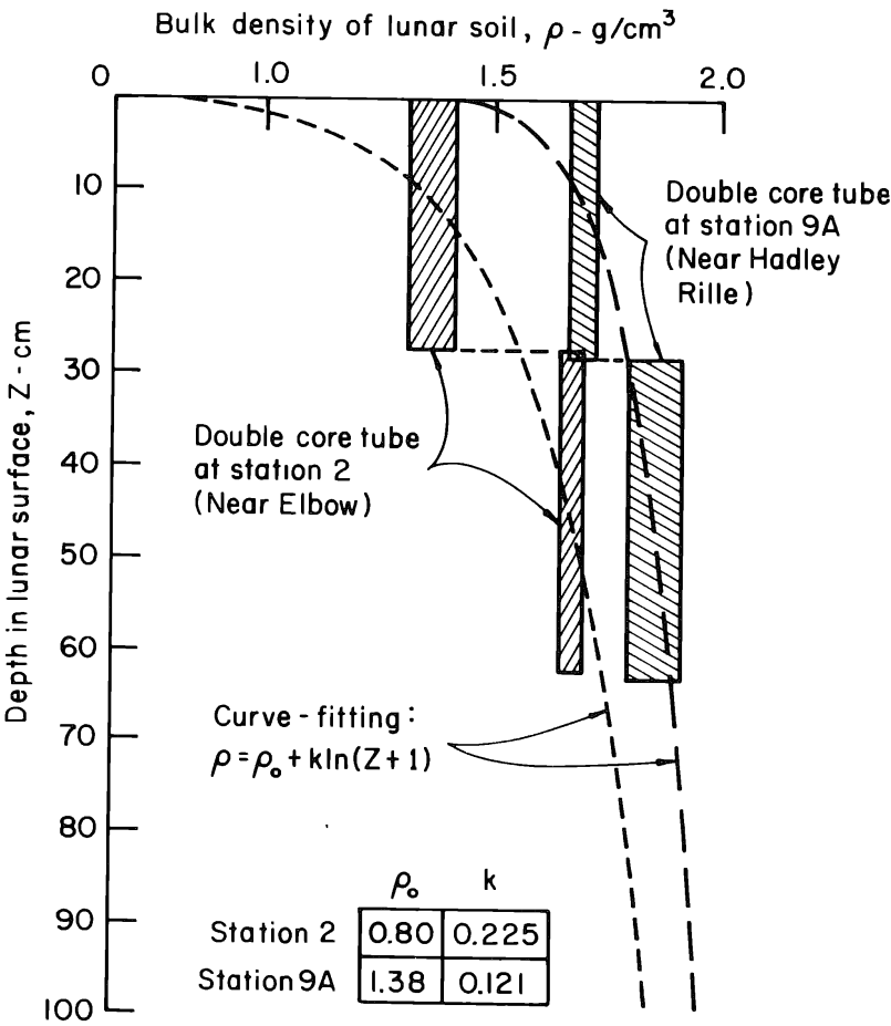
Fig. 6. Density of lunar soil at Apollo 15 core tube sites.
