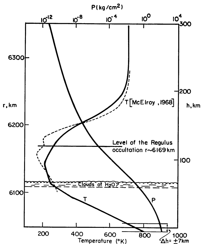
Fig. 1. Structure of the Venus atmosphere as determined from Veneras 5 and 6. This diagram is redrawn from one in the paper by Avduevsky et al. , 1970 (and with the addition of the question mark in the clouds).
