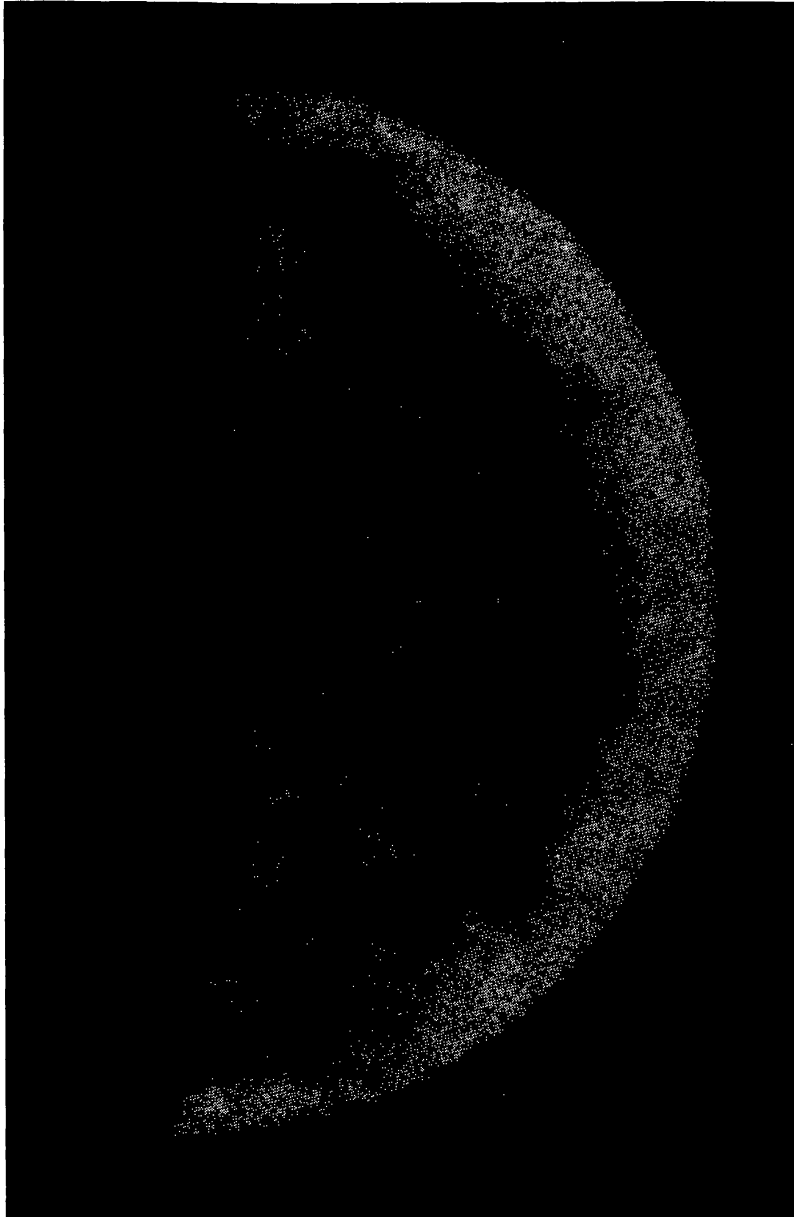
Fig. 2. An unusual drawing of Venus by J. H. Focas showing apparent resolution of the clouds into individual elements [taken from Atlas des Planètes (ed. by V. de Callataj and A. Dollfus), Gauthier-Villars, Paris, 1968].
