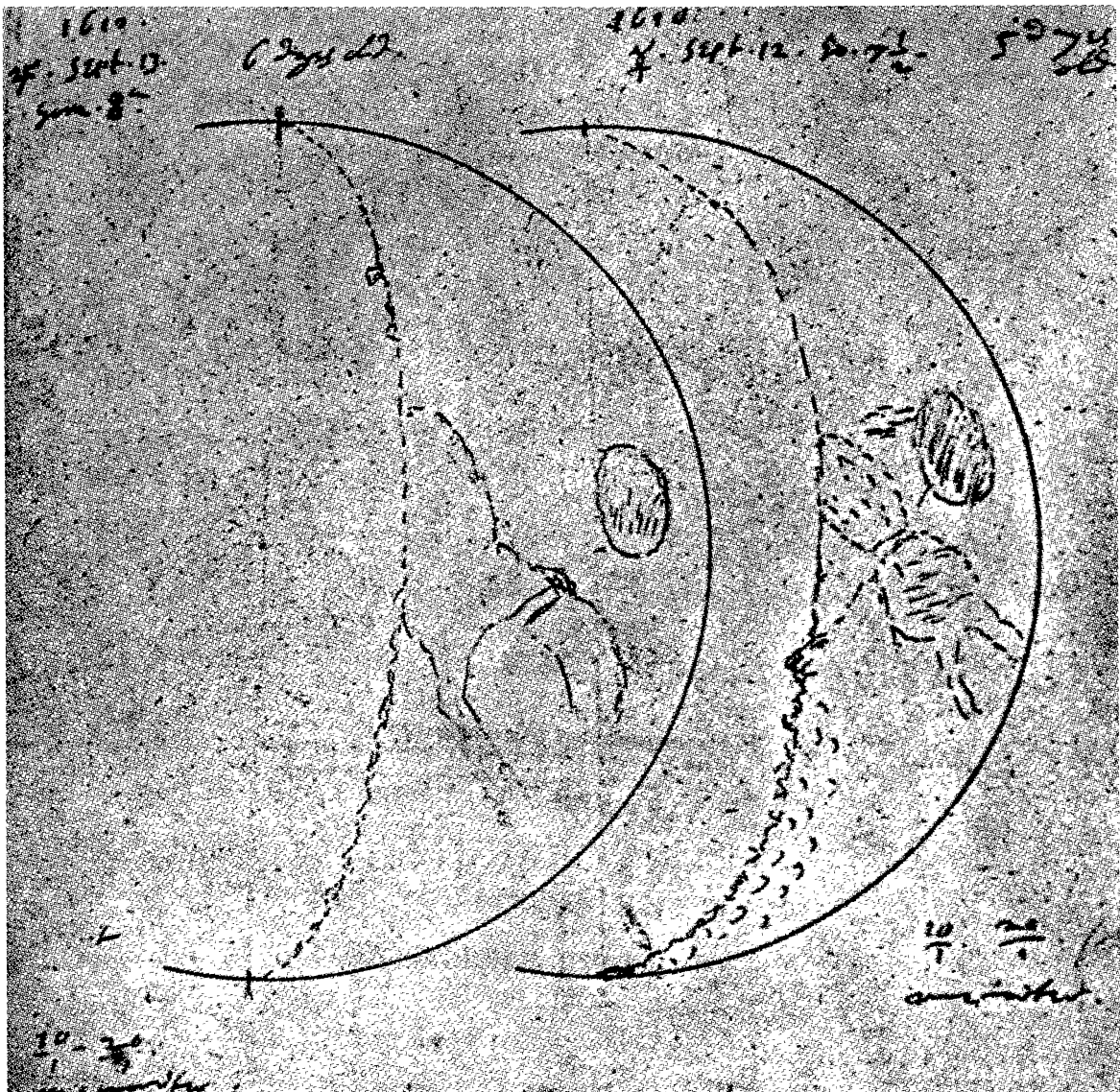
Fig. 3. Two of the drawings of the waxing Moon by Thomas Harriott, dated 1610 September 12 and 13, based on telescopic observations, and showing clearly Mare Crisium as well as what appears to be outlines of Mare Tranquillitatis and Nectaris.
