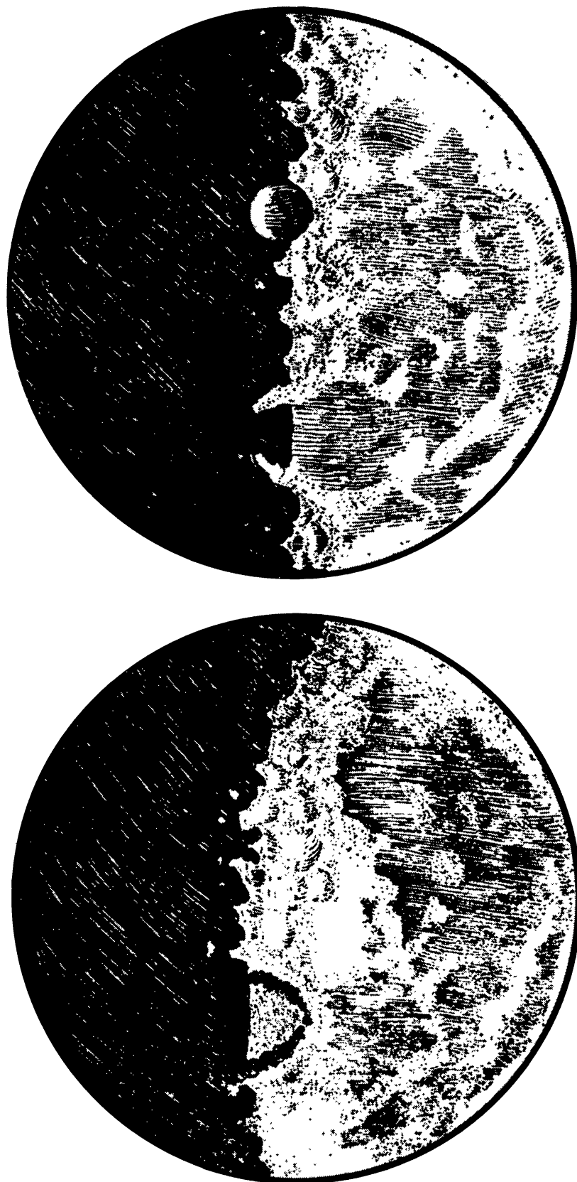
Fig. 2. Two of the four drawings of the Moon made by Galileo Galilei and reproduced in his Sidereus Nuncius (Venice, 1610; also on p. 67 of vol. 3, 1 of his Edizione Nazionale, 1964). The drawings reproduce apparently but schematized views of what Galileo saw with his telescope; for none of the features recorded on them can be identified with certainty with any known formation.
