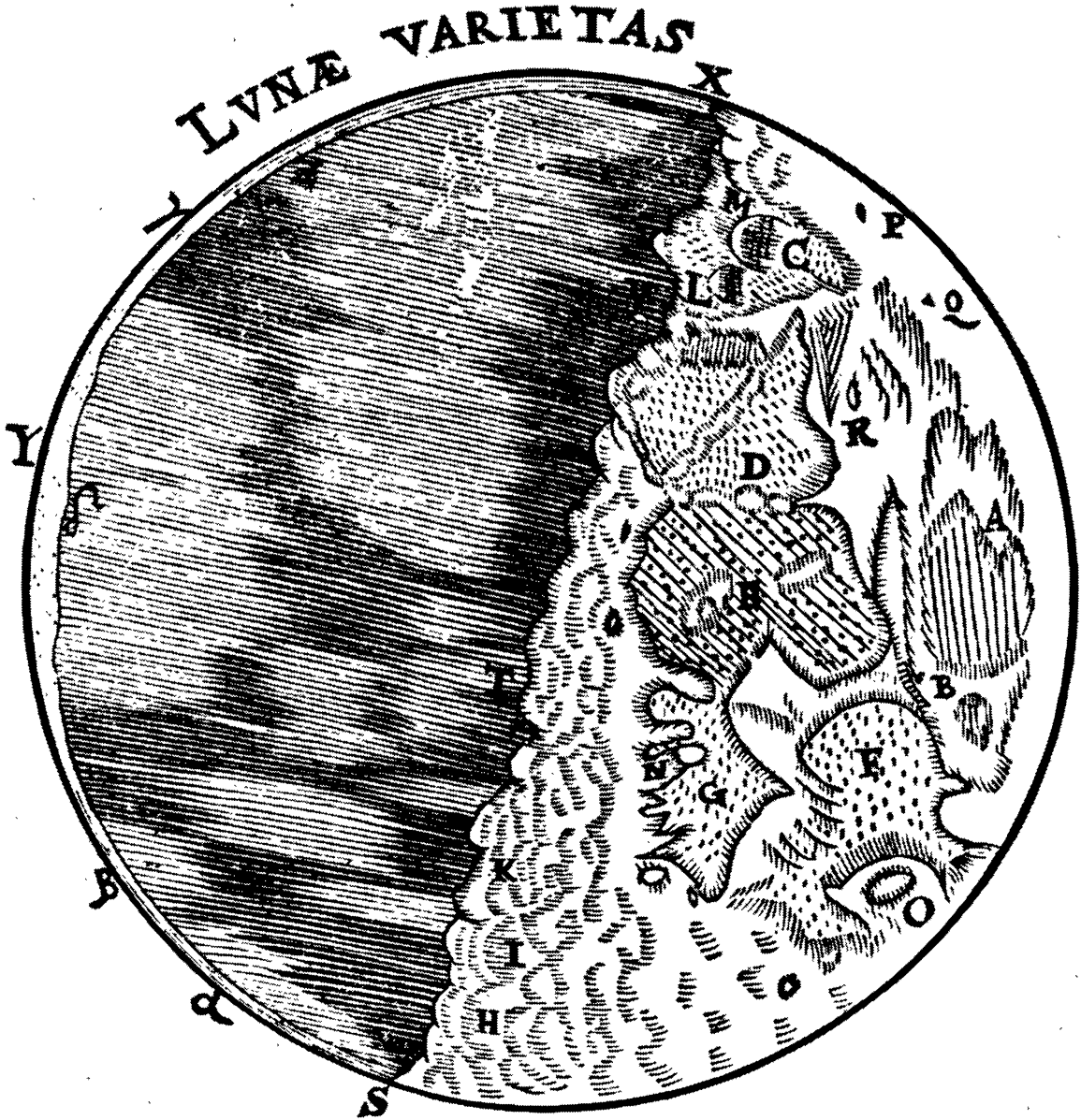
Fig. 5. A drawing of the first quarter of the Moon, prepared by Christoph Scheiner probably before 1613, and published a year later in Disquisitiones Mathematicae . Some of the surface features labelled by letters can be readily identified. Thus A denotes Mare Crisium; E, Mare Tranquillitatis; F, Mare Foecunditatis; G, Mare Nectaris; and M, the crater Aristoteles. Like on all drawings reproduced on Figures 1–4, North is on top (as the Moon is seen by the naked eye, or the Galilean telescope). As Scheiner is known to have used the Keplerian (inverting) telescopes since 1613, it is believed that the drawing reproduced above was made before that time.
