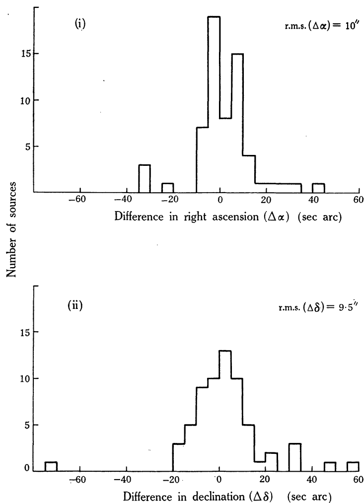
Fig. 5.—Histograms of differences between optical and radio positions for quasi-stellar objects, in (i) right ascension and (ii) declination.
