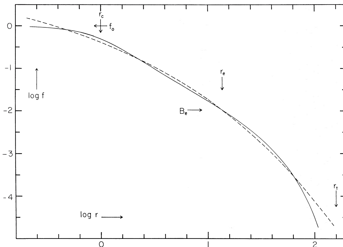
FIG. 5. Comparison between de Vaucouleurs' law and a modified isothermal model. Characteristic parameters of each curve are marked.
