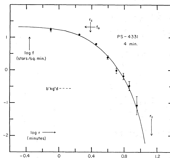
FIG. 3. Comparison of star counts in NGC 5053 with theoretical curve for \log(r_t/r_c)=0.75 . Medium-exposure 48-in. Schmidt plate.
