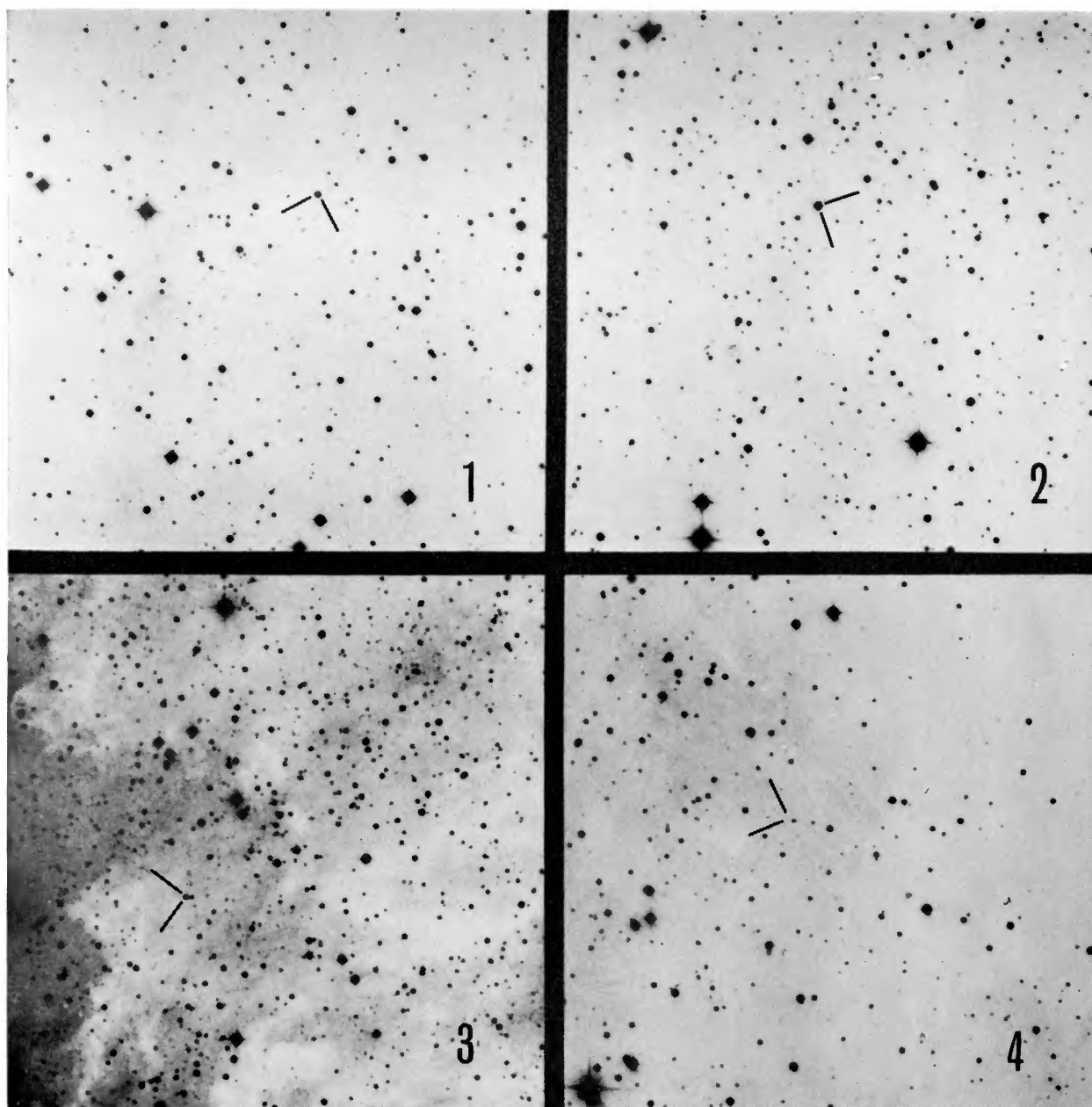
FIG. 3.—Finding charts Nos. 1-4 for Haro-Chavira objects
