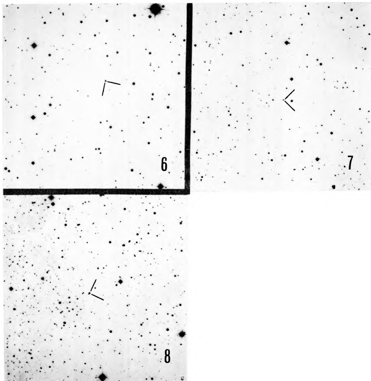
FIG. 4.—Finding charts Nos. 6–8 for Haro-Chavira objects
