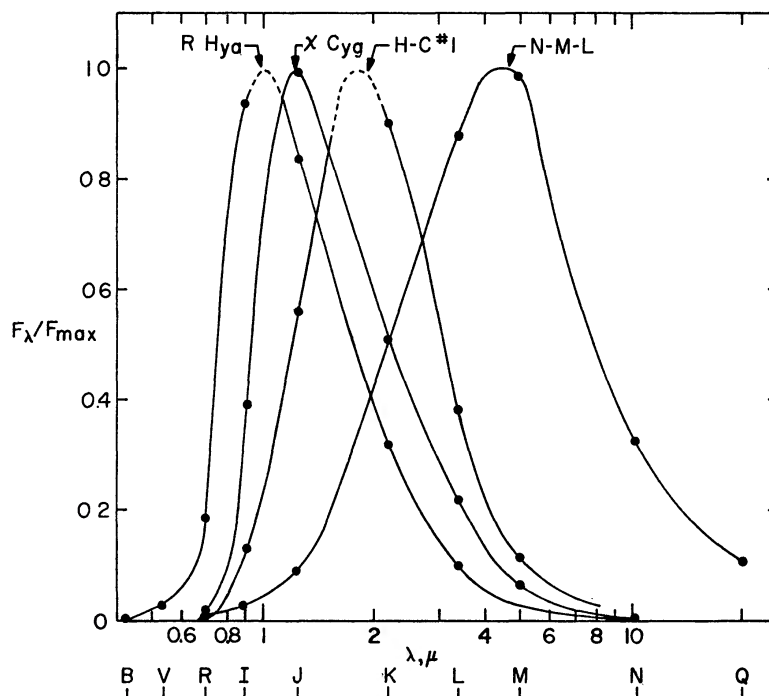
FIG. 1 —The spectral-energy curves for R Hya, \chi Cyg, Haro-Chavira 1, and the Neugebauer-Martz-Leighton Cygnus object.
