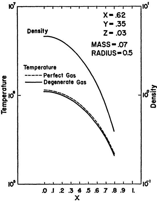
FIG. 2.—The temperature and density distributions in a completely convective model
