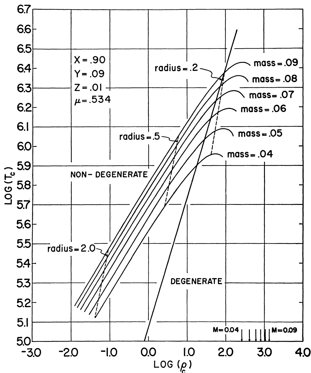
FIG. 4.—The temperature-density diagram for completely convective models. Population II
