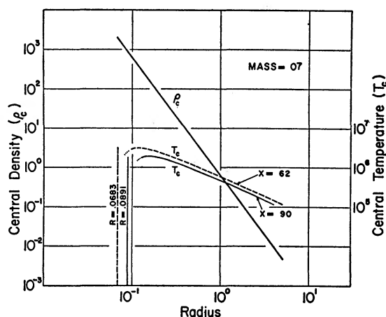
FIG. 1.—The central temperature and the central density in completely convective models
