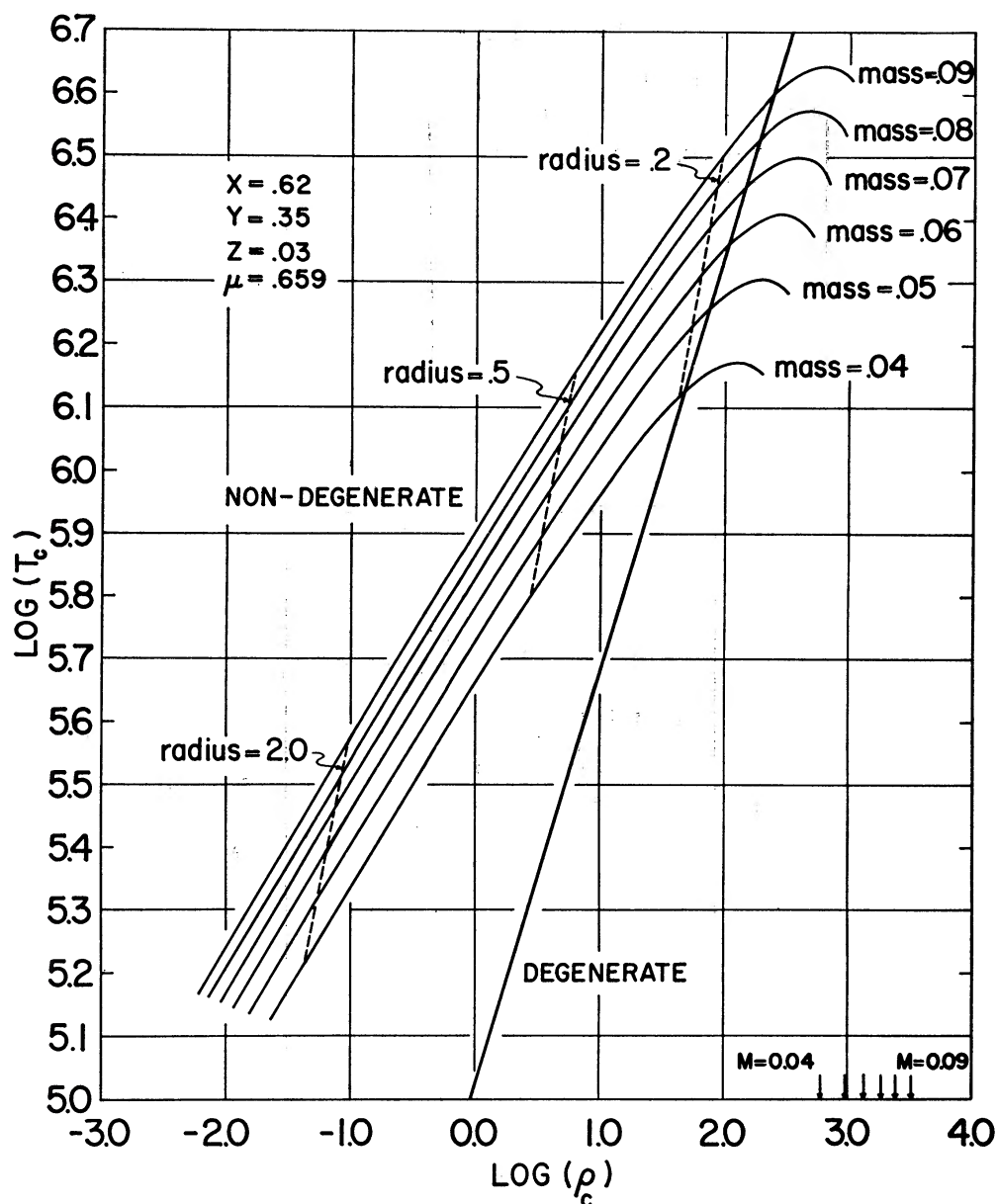
FIG. 3.—The temperature-density diagram for completely convective models. Population I
