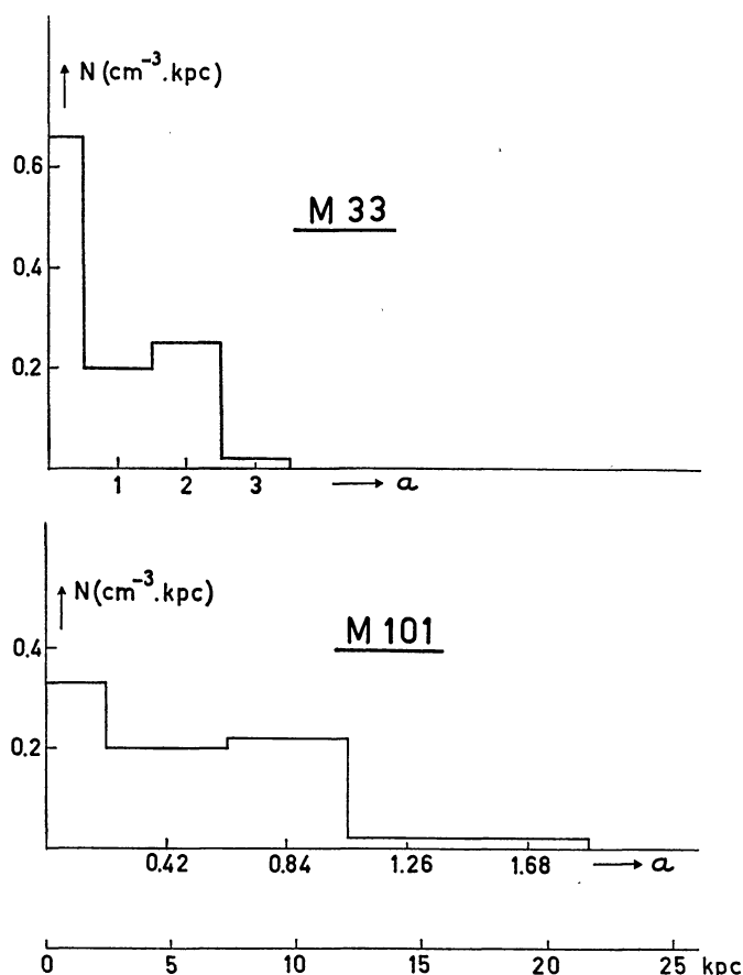
Density distribution in M33 and M101.
