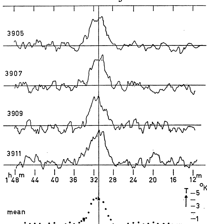
Four drift curves and their mean at \delta = 30^\circ 17' and V = -148 km/sec with respect to L.S.R. The squares are obtained by interpolation from Figure 1b.
