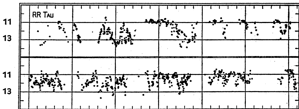
Figure XI, 2.—Observations of RR Tauri, (between J.D. 2425000 and 2431000) made by the A.A.V.S.O. and other groups of observers. The magnitudes were compiled by Mr. Campbell, and are used here with his kind permission.
