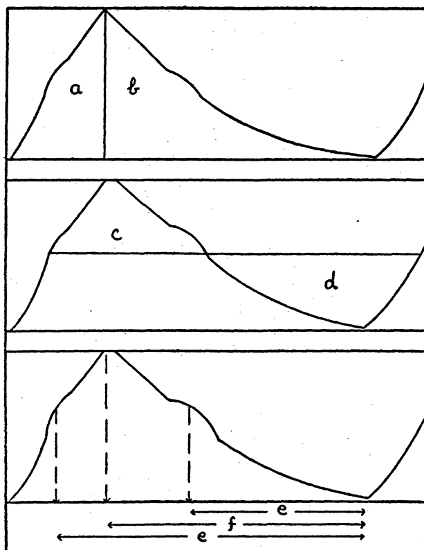
Figure III, 1.—Parameters for describing the light curve: a/b , c/d , and e/f . From S. Gaposchkin, P.N.A.S., 24, 1, 1938.
