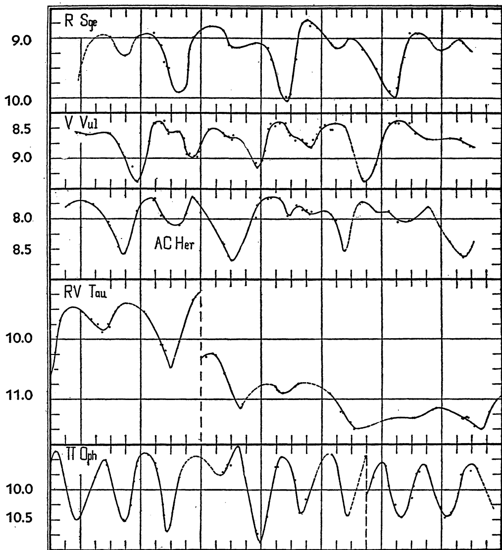
Figure V, 1—Typical “RV Tauri” stars:
