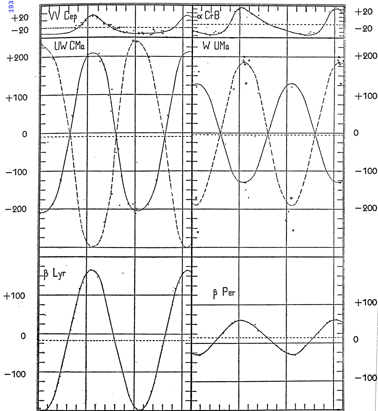
Figure II, 2.—Velocity curves for six eclipsing stars. Abscissae are as in Figure II, 1, for the five stars common to the two figures; short vertical lines indicate intervals of one tenth of the period. Ordinates are kilometers per second, as indicated in the margins. Sources of data are as follows: VV Cephei, S. Gaposchkin, H.C. 421, 1938 (single observations). \alpha Coronae Borealis, Jordan, Publ.Allegh.Obs., 1, 91, 1909. UW Canis Majoris, Pearce, Publ.Dom.Ap.Obs., 6, 51, 1932; Luyten and Ebbighausen, Ap.J., 82, 247, 1935. W Ursae Majoris, Adams and Joy, Mt.W.Contr., 8, 358, 1919. \beta Lyrae, Rossiter, Publ.Mich.Obs., 5, 88, 1933. \beta Persei, McLaughlin, Publ. Mich.Obs., 6, 3, 1934.
