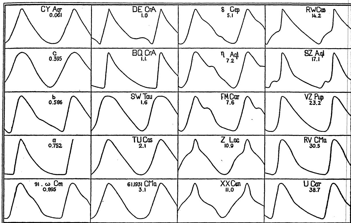
Figure IV, 1—Mean photographic light curves for typical Cepheid variables, arranged in order of period. All are reduced to the same scale, both of ordinates and of abscissae. Sources of the light curves are as follows: CY Aquarii, S. Gaposchkin, H.B. 898, 1935. Cluster type variables of Bailey's classes c, b, and a, Shapley, Star Clusters , p. 54, 1930. Star No. 91 in \omega Centauri, Bailey, H. A., 38, 2, 1902. DE and BQ Coronae Austrinae, B.A.N. 243, 1933. SW Tauri, TU Cassiopeiae, XX Centauri, Robinson, H. A., 90, No. 2, 1932. 61. 1931 Canis Majoris, VZ Puppis, RV Canis Majoris, Florja, Publ. Sternberg Astr. Inst. No. 8, 1937. \delta Cephei (photoelectric), Stebbins, see Russell, Dugan, and Stewart, p. 760, 1927. \eta Aquilae, (photoelectric), Wylie, see Handbuch d. Ap. 6, 189, 1928. FM Carinae, Z Lacertae, RW Cassiopeiae, and U Carinae, Hertzsprung, B.A.N. 96, 1926.
