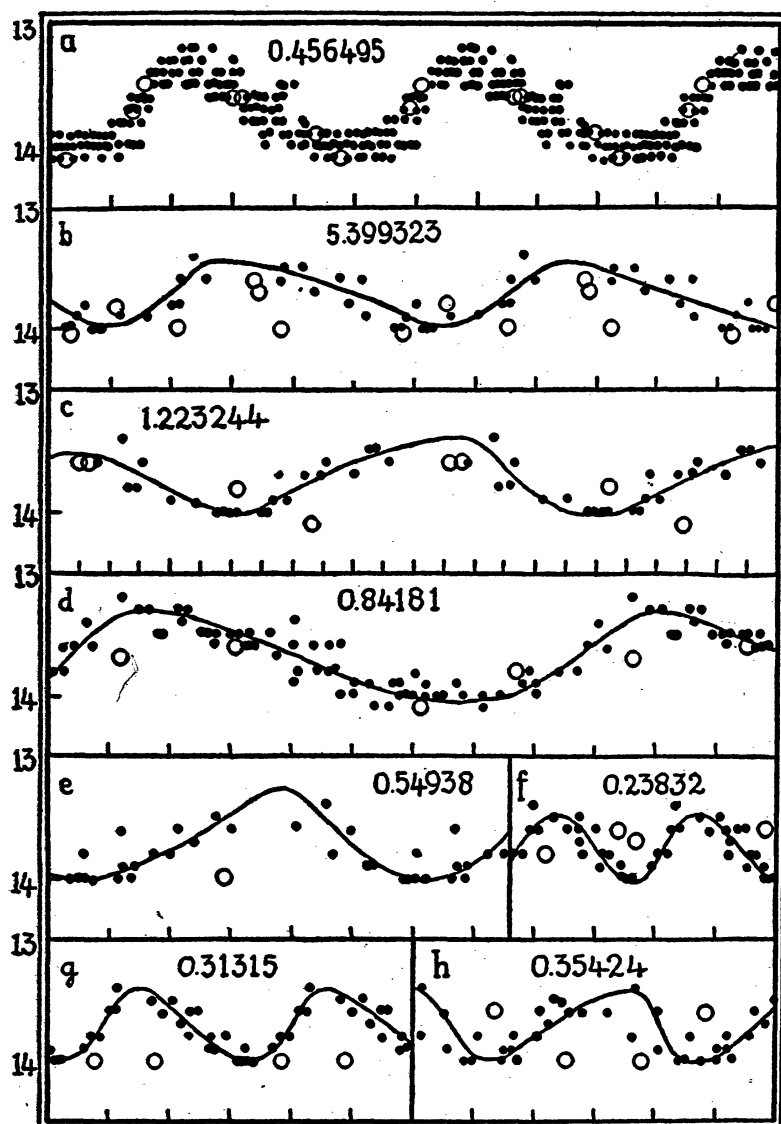
Figure XII, 1.—Observations of the cluster type variable QV Centauri, discussed with the correct period (a) and with seven spurious periods, related as follows (for notation, see text):
