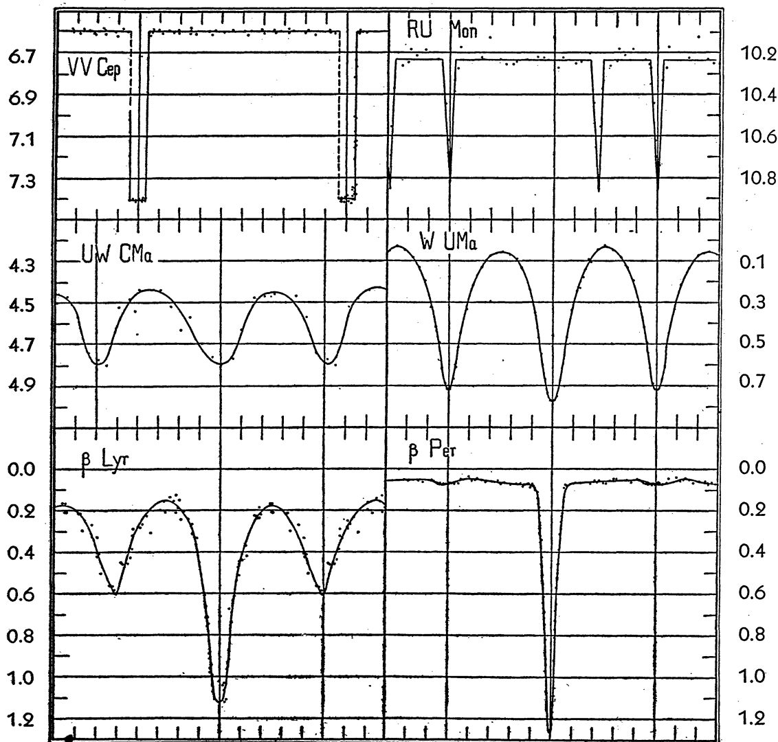
Figure II, 1.—Light curves for six eclipsing stars. Abscissae are phases (short vertical lines indicate intervals of one tenth of the period). Ordinates are magnitudes, as indicated in the margins. Sources of data are as follows:—VV Cephei, S. Gaposchkin (H.C. 421, 1938, and unpublished); the minima shown are those of 1915-1916 and 1936-1937. RU Monocerotis (visual observations), Dubiago, A.N., 235, 235, 1928. UW Canis Majoris (photographic observations), S. Gaposchkin, H.B. 902, 1936. W Ursae Majoris (photoelectric observations, relative magnitudes), C. M. Huffer, Ap.J., 79, 375, 1934. \beta Lyrae (photoelectric observations, relative magnitudes), Smart, M.N., 95, 648, 1935. \beta Persei (photoelectric observations, relative magnitudes), Smart, M.N., 97, 403, 1937.
