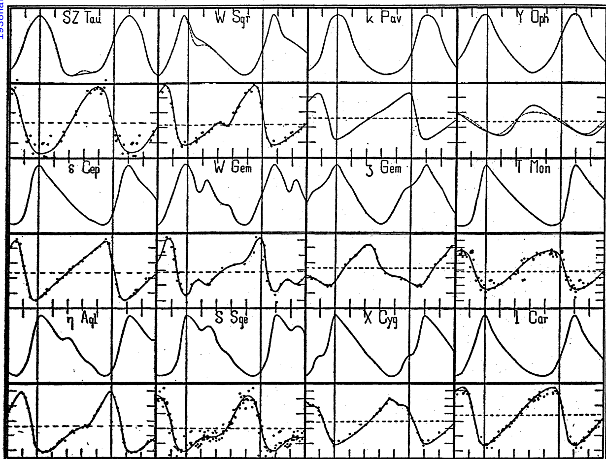
Figure IV, 2.—Comparison of light curves and velocity curves for twelve typical Cepheid variables. All light curves are reduced to the same scales of ordinates and abscissae. Velocity curves are all reduced to the same scales of abscissae; short horizontal lines on the left and right indicate intervals of 10 kilometers per second in radial velocity. Broken horizontal lines indicate the systemic velocities as follows: SZ Tauri, -3.15 km/sec; \delta Cephei, -16.83 km/sec; \eta Aquilae, -14.16 km/sec; W Sagittarii, -28.6 km/sec; W Geminorum, -0.70 km/sec; \kappa Pavonis, +36.5 km/sec; \zeta Geminorum, +6.8 km/sec; X Cygni, +9.32 km/sec; Y Ophiuchi, -6.1 km/sec; T Monocerotis, +4 km/sec; I Carinae, +4.08 km/sec.
