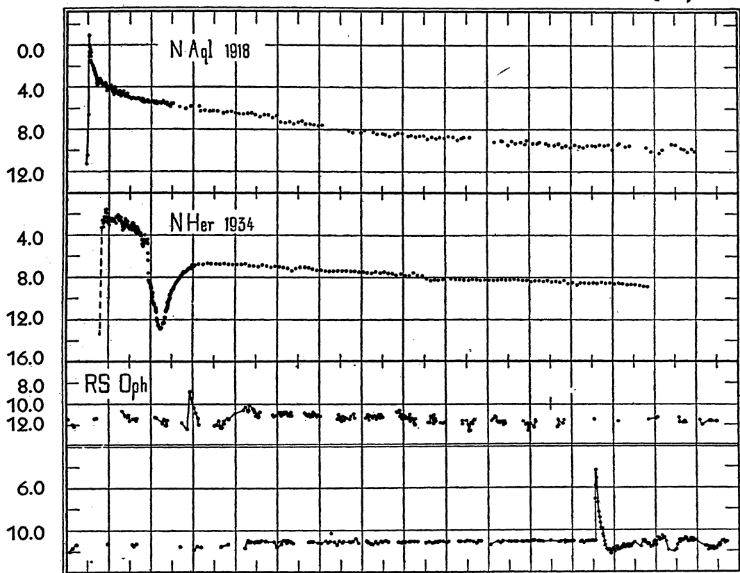
Figure VII, 1.—Light curves of three novae of different types:
