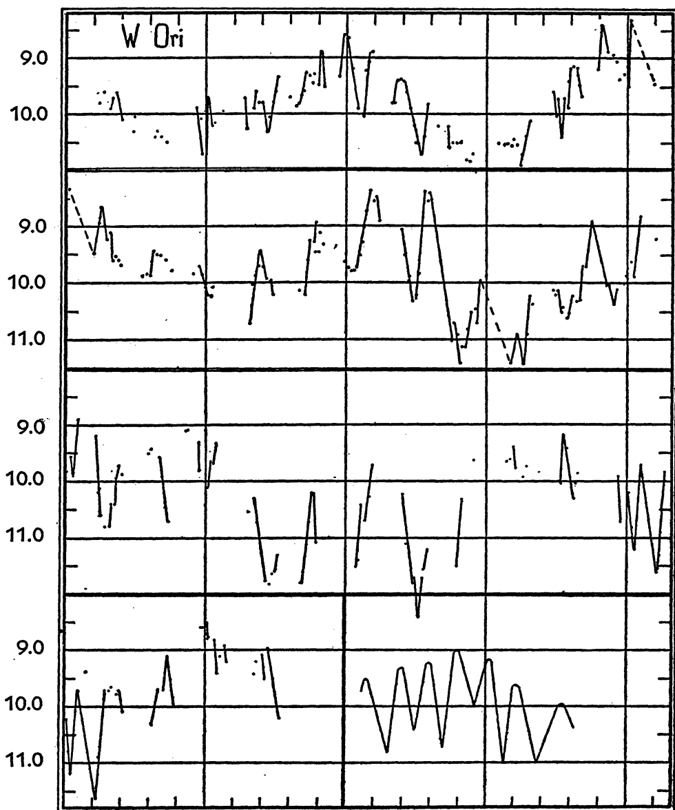
Figure III, 5.—Variations of W Orionis. The observations are photographic estimates made on Harvard plates. Abscissae are Julian Days (short vertical lines indicate intervals of 200 days, vertical cross-lines, intervals of 1000 days). The observations cover the interval from J.D. 2414000 to J.D. 2428000. In the lower right corner is the mean light curve for the whole interval, showing the long-term variation (short vertical lines indicate intervals of 2000 days, vertical cross-lines, intervals of 10,000 days). Ordinates are photographic magnitudes, as indicated in the margin.
