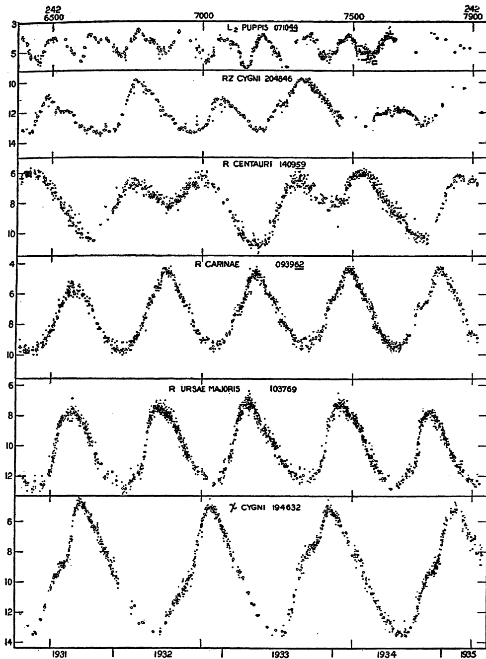
Figure III, 3.—Light curves of six long-period variables, from visual observations made by the A.A.V.S.O. and other groups of observers. From Campbell, Harv. Repr. 132, 1937; reproduced with his permission.
