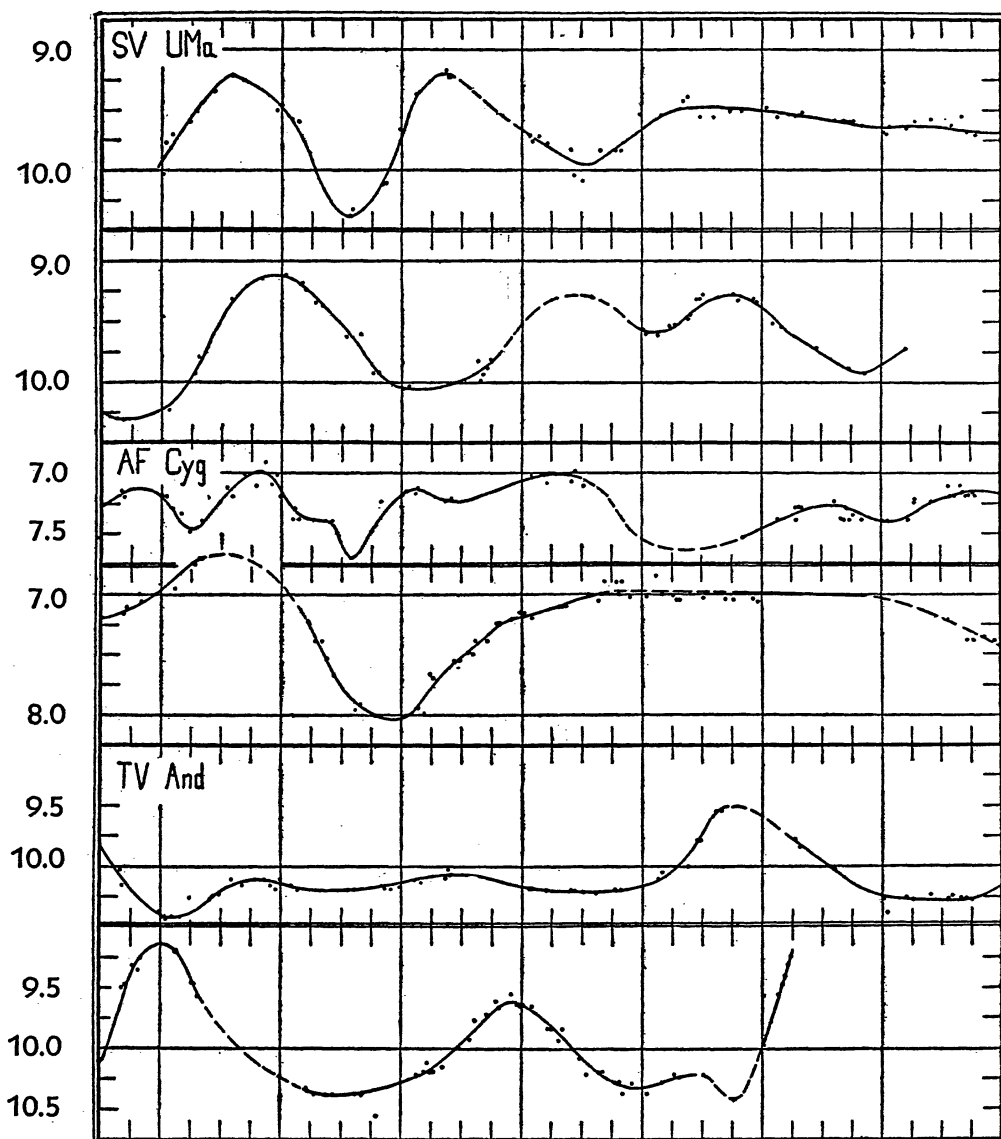
Figure V, 3.—Typical “long-period” semiregular variables:
