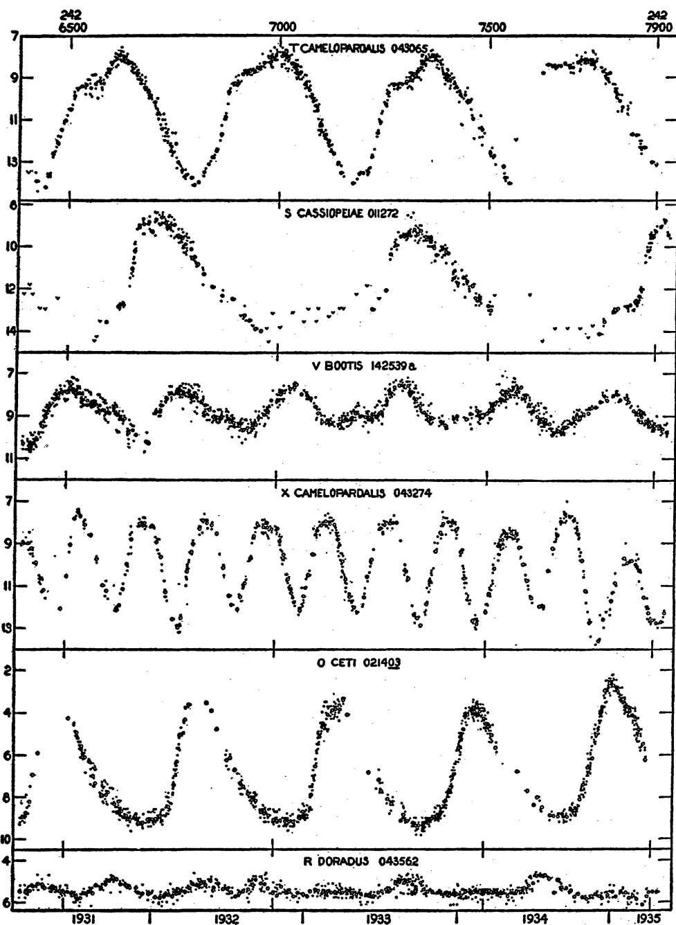
Figure III 2.—Light curves of six long-period variables, from visual observations made by the A.A.V.S.O. and other groups of observers. From Campbell, Harv. Repr. 132, 1937, reproduced with his kind permission.
