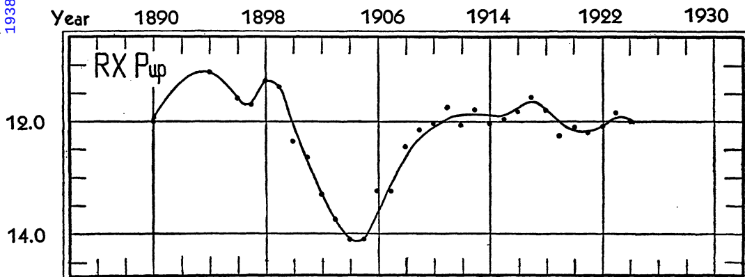
Figure XI, 1.—Light curve of RX Puppis, from photographic observations made on Harvard plates.
