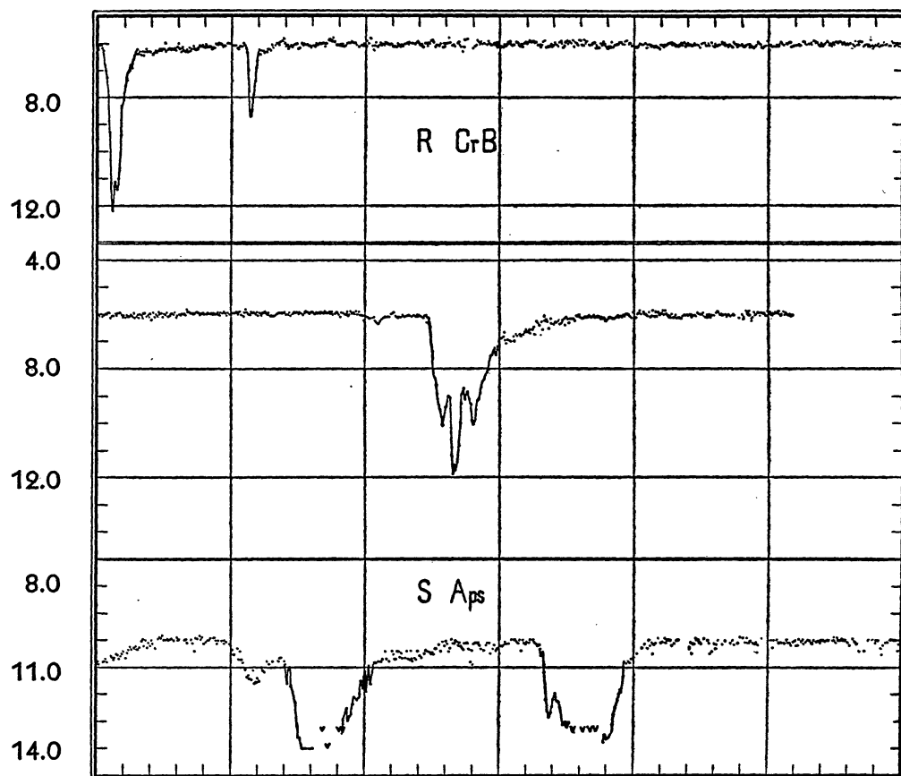
Figure X, 1.—Light curves of “R Coronae Borealis” stars: R Coronae Borealis between J.D. 2423500 and 2429500 S Apodis between J.D. 2426000 and 2429000
