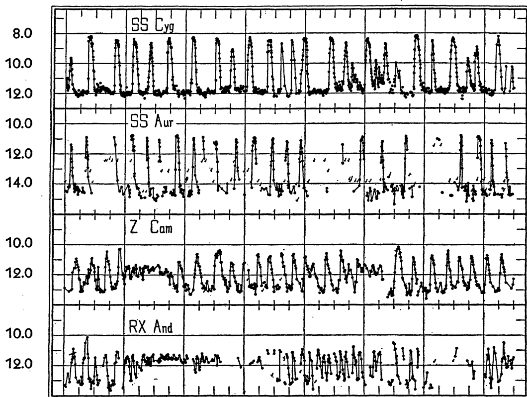
Figure IX, 1.—Light curves of "SS Cygni" variables:
