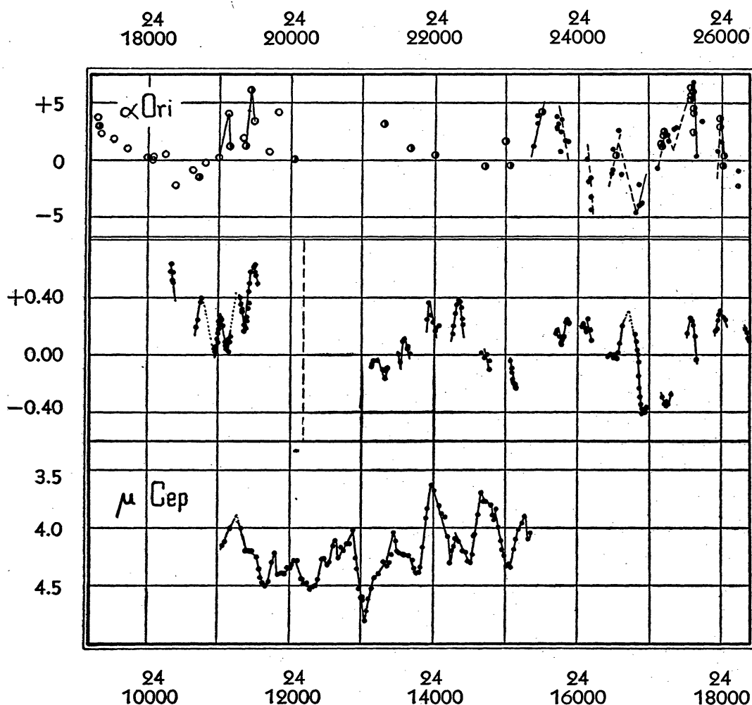
Figure V, 6.—Typical “ \mu Cephei” stars:
