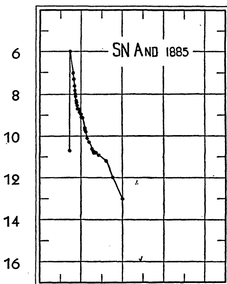
Figure VIII, 1.—Light curve of the supernova S Andromedae, compiled from various sources by Mr. Campbell, with whose kind permission it is reproduced. The observations cover the interval from J.D. 2409700 to J.D. 2410100.
