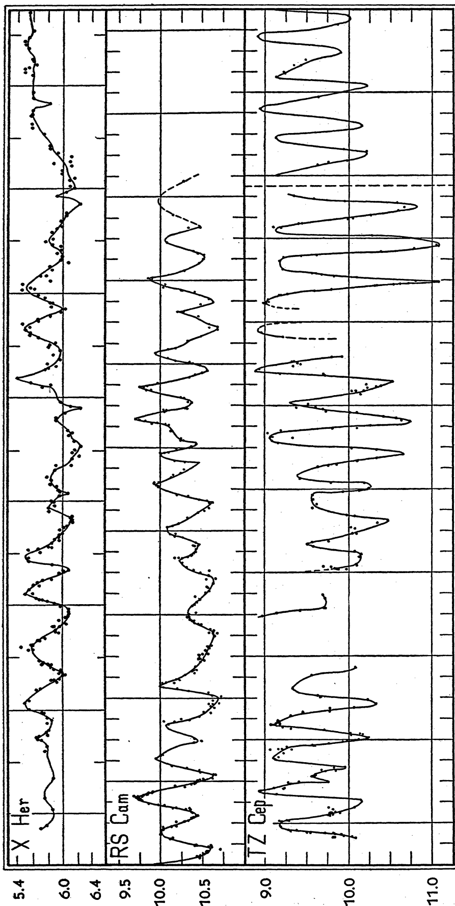
Figure VI, 1.—Typical irregular red variables:
