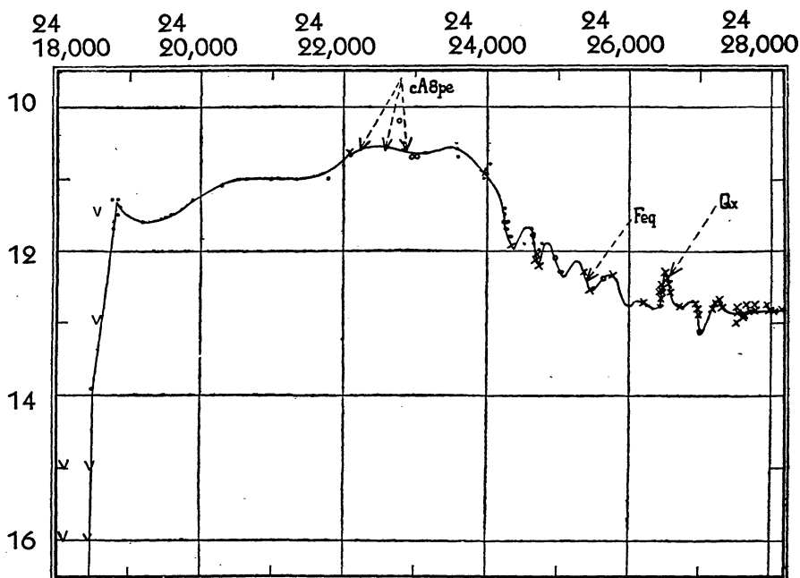
Figure VII, 2.—Light curve of Nova (RT) Serpentis 1909. Dots represent published photographic observations (Shapley, P.A.S.P., 31, 230, 1919; Bailey, H.B. 753, 1921; Shapley, H.B. 789, 1923). Circles represent published visual observations, as follows: (Graff, B.Z., p. 55, 1921; ib. , No. 25, 1922; ib. , No. 12, 1927; Lacchini, B.Z., p. 59, 1921; ib. , No. 5, 1929; A.N., 248, 366, 1933). Crosses represent unpublished Harvard observations. The arrows refer to points on the light curve at which spectroscopic observations have been made.
