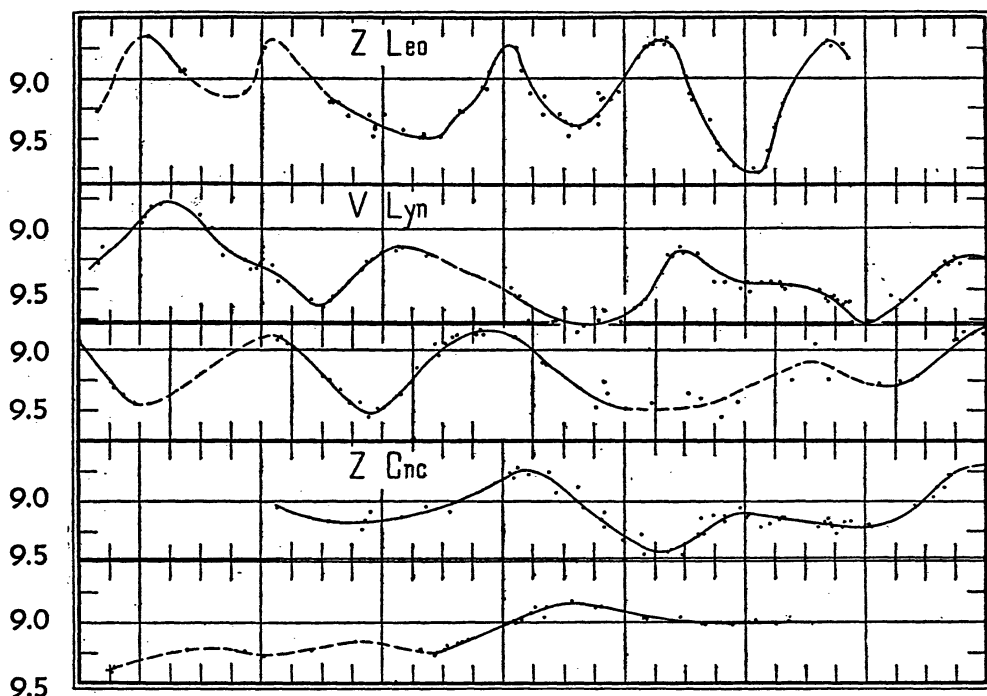
Figure V, 5.—Typical “UU Herculis” stars:
