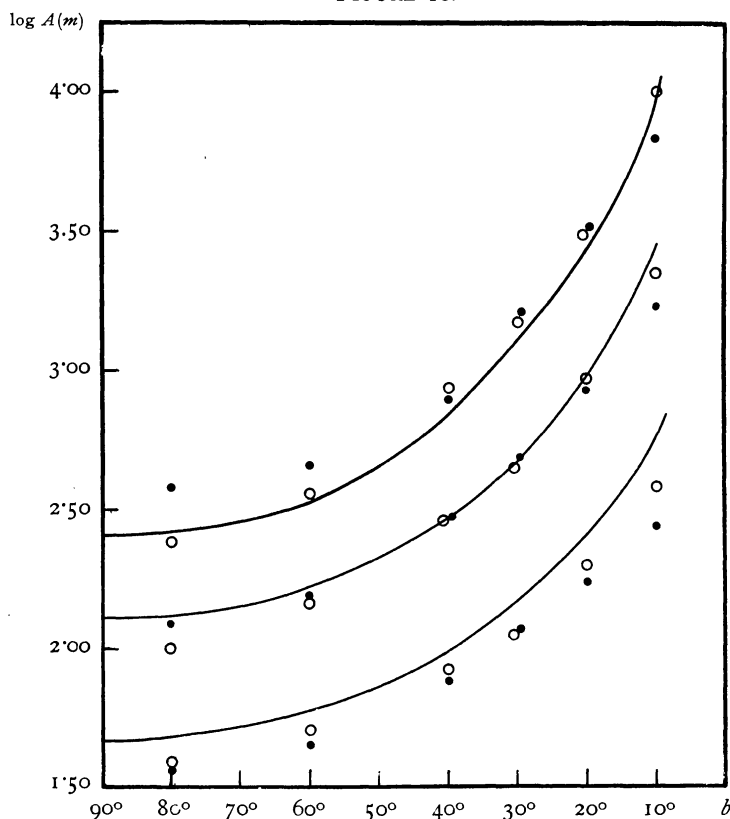
Relation between observed and computed numbers of stars at different galactic latitudes.
