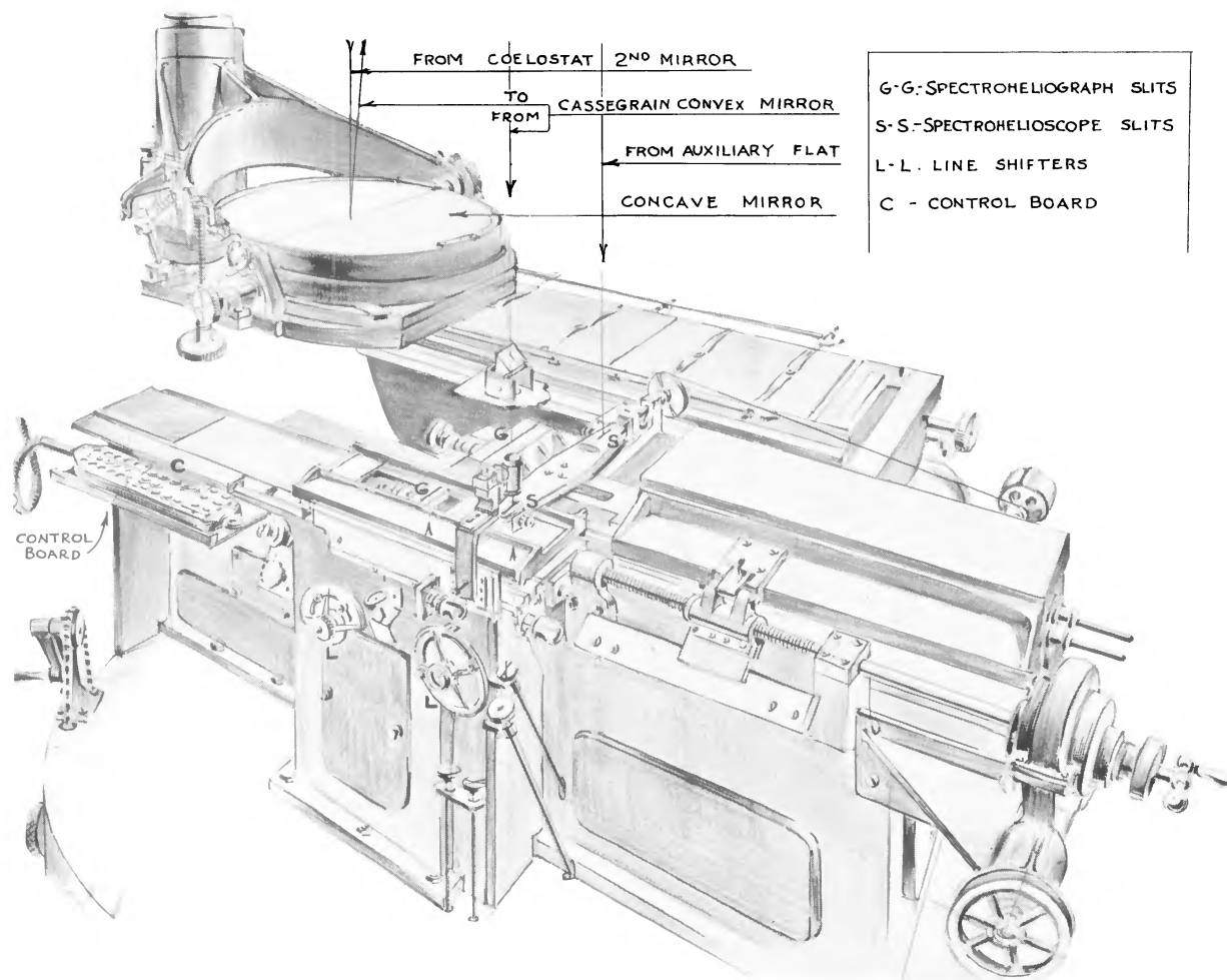
COMBINED SPECTROGRAPH, SPECTROHELIOGRAPH, AND SPECTROHELIOSCOPE
