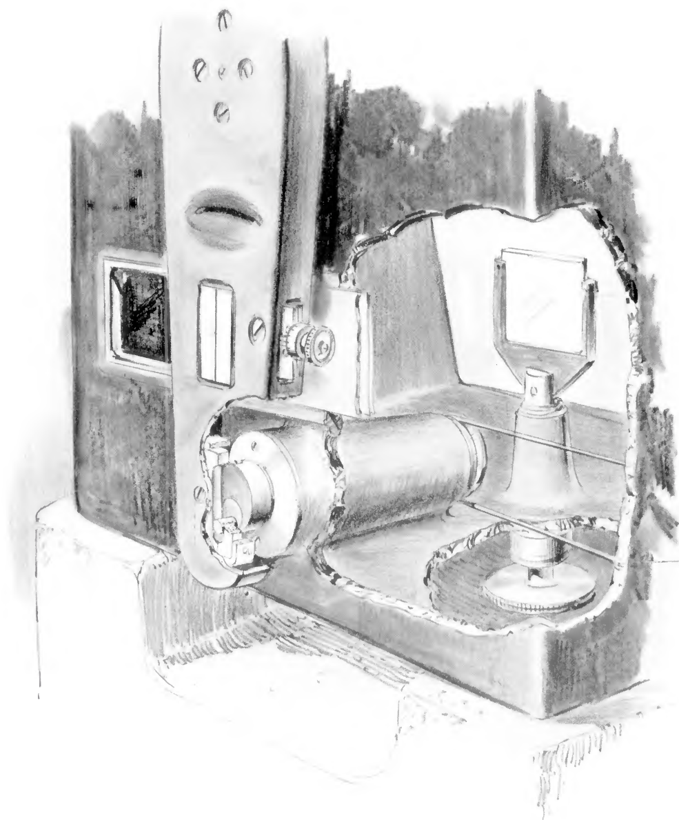
SECOND SLIT, DRIVING MECHANISM, AND LINE-SHIFTER
