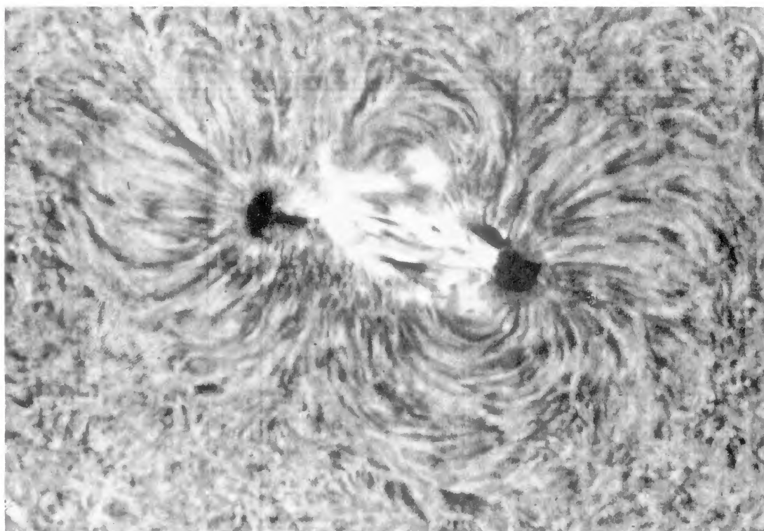
d. —Structure of hydrogen flocculi near large bipolar sun-spot group of August 30, 1924. From a spectroheliogram by Lewis Humason.
