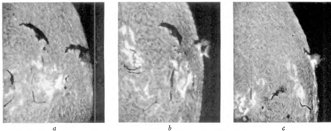
a, b, c. —Hydrogen flocculi photographed on three successive days. From spectroheliograms taken by A. H. Joy on June 27, 28, and 30, 1916.
