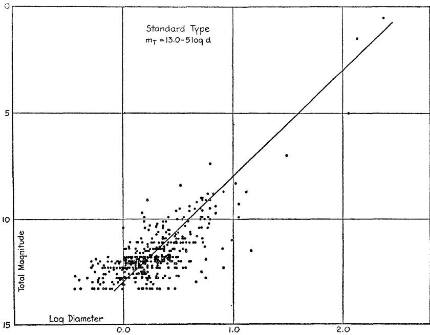
FIG. 7.—Relation between luminosity and diameter among extra-galactic nebulae. The nebulae have been reduced to a standard type, S_0 , which, being the mean of E_7 , S_a , and S_{Ba} , represents a hypothetical transition point between elliptical nebulae and spirals. The Magellanic Clouds have been included in order to strengthen the brighter end of the plot.
