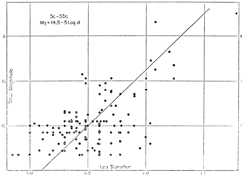
FIG. 4.—Relation between luminosity and diameter among nebulae at the end of the sequence of types—Sc and SBc nebulae.
