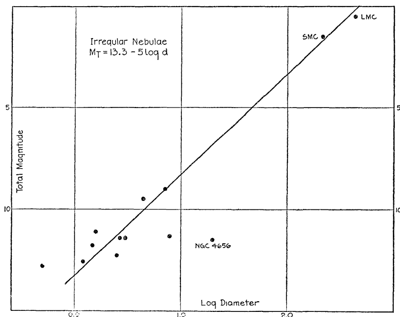
FIG. 5.—Relation between luminosity and diameter among the irregular nebulae. The Magellanic Clouds are included. N.G.C. 4656 is an exceptional case in that it shows a narrow, greatly elongated image in which absorption effects are very conspicuous; hence the maximum diameter is exceptionally large for its apparent luminosity.
