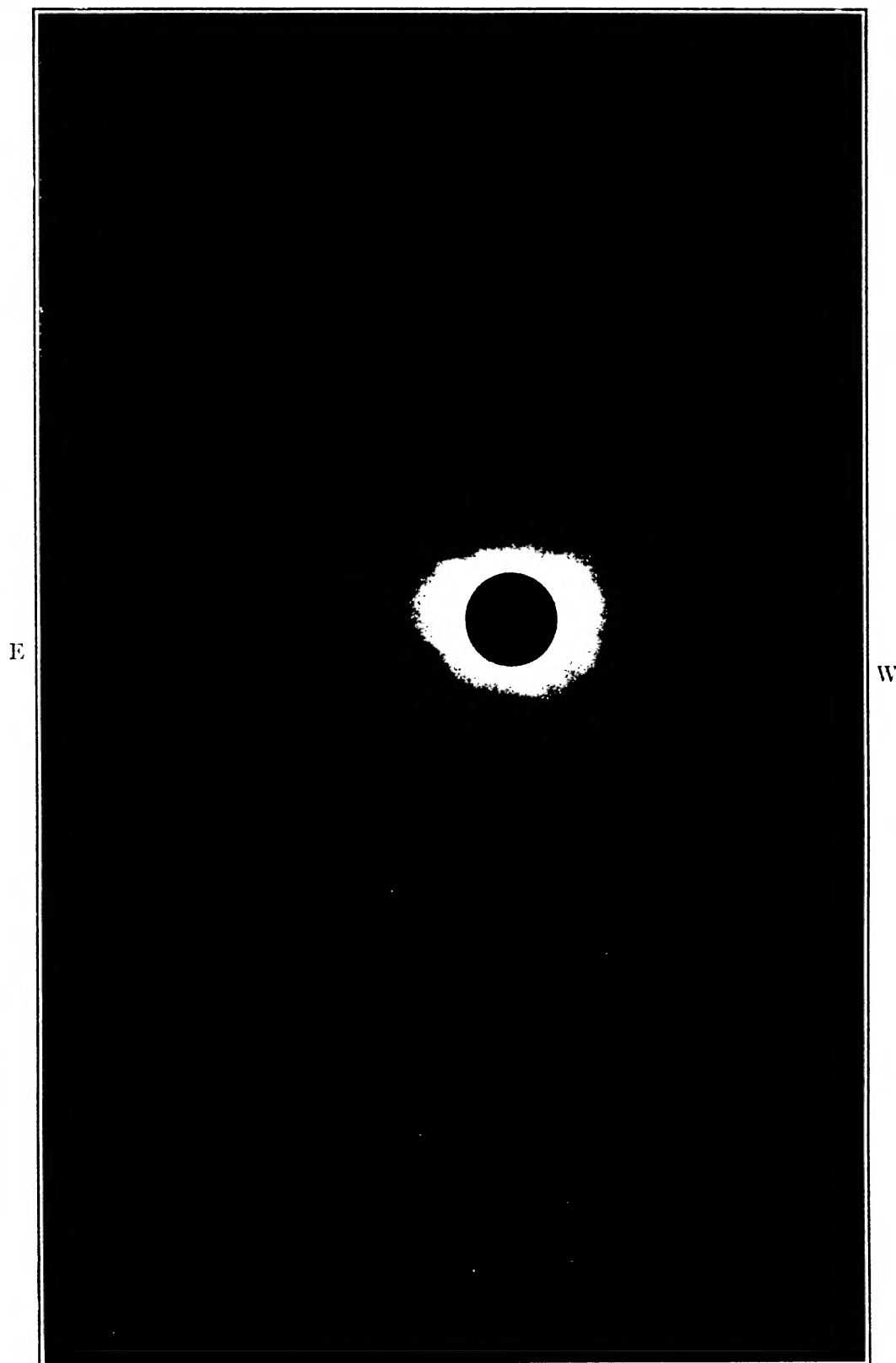
FIG. 4. THE SOLAR CORONA (Focal length of camera, 48 inches)
