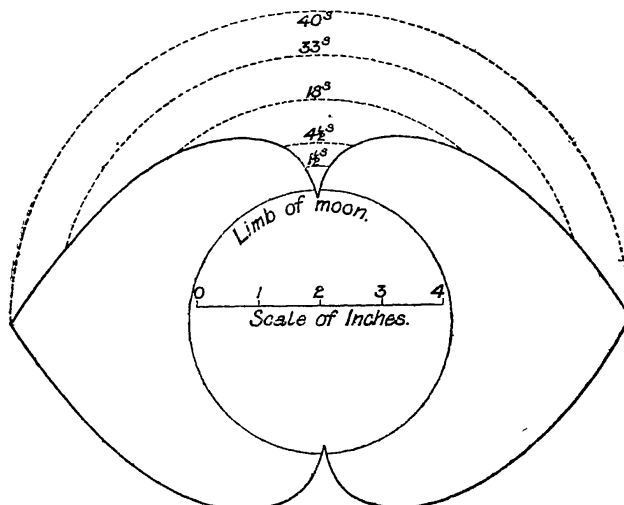
The figures against the dotted lines show the effective exposures at different distances from the Sun's centre.
