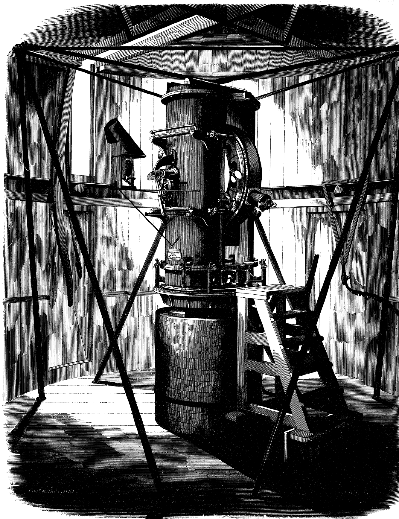
A PERSPECTIVE VIEW OF THE ALTITUDE AND AZIMUTH INSTRUMENT,
