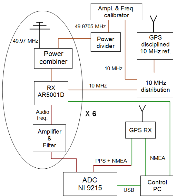
Figure 4 – Schematic of the interferometer in Humain.
