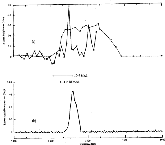
Figure 6: Optical and radio flaring of V371 Orionis on 30 November 1962. (a) Optical light curves (solid line = Baker-Nunn photographs; dashed line = amateur observations). (b) Smoothed line = 410 MHz Parkes plot; time intervals with 19.7 MHz (Fleurs) and 1410 MHz (Parkes) emission are also indicated (after Slee, Solomon, and Patston, 1963: 993).
