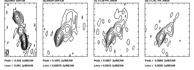
Fig. 4. (a) Self-calibrated Image for J0842. Images for J0839: (b) Self-calibrated Image; (c) 2-cal phase referencing; (d) 1-cal phase referencing.
