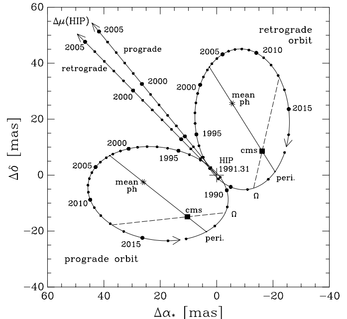
Fig. 1. Astrometric orbit (prograde or retrograde) of the photo-center of \alpha UMi AP. The retrograde orbit is our preferred solution. For detailed explanations see Sect. 3.2.4
