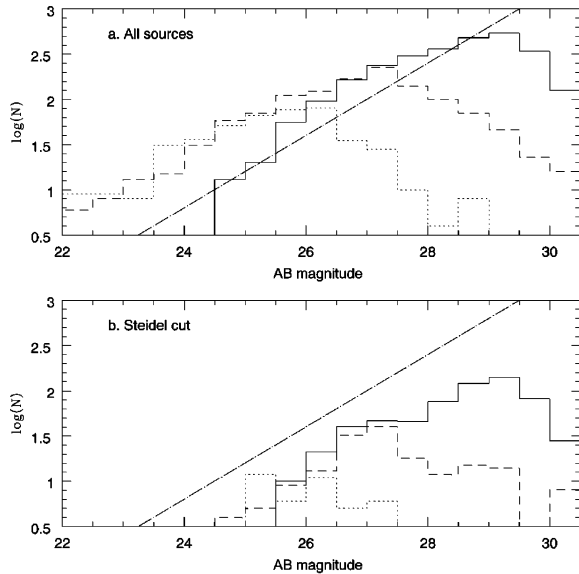
FIG. 2.—Number-magnitude relations in catalogs derived from unsmoothed data (solid lines), 0".5 smoothed data (dotted lines), and 1".0 smoothed data (dashed lines): (a) the full catalogs and (b) the high color-redshift subset only. In (a) the completeness limit decreases by 2 and 4 mag after smoothing, while the number counts decrease by factors of 2 and 4, respectively. The dot-dashed line has slope 0.4.
