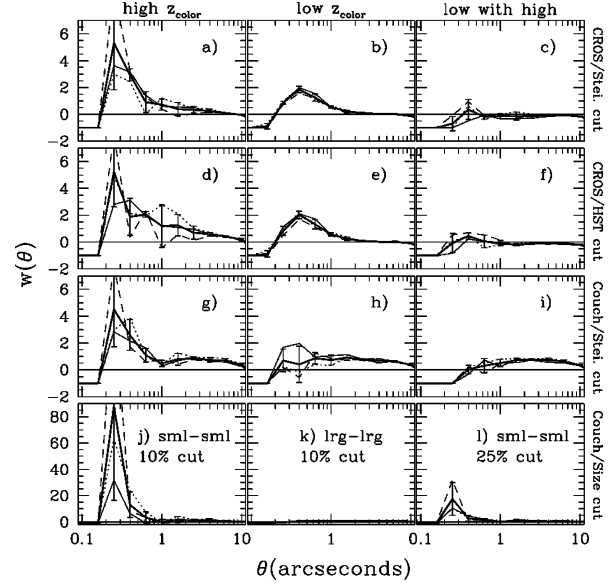
FIG. 1.—Angular correlation for WFC chips 2, 3, and 4 of the Hubble Deep Field. The lighter curves ( solid , dotted , and dashed , respectively) are for the individual chips. The heavier curve is the mean of those three values. In the first three rows, three different catalogs and color-redshift cuts are plotted in each column. The top row (a)–(c) is for our catalog with the Steidel color-redshift cut. The middle row (d)–(f) is for our catalog with the HST cut (see text). The third row (g)–(i) is for the Couch catalog with the Steidel cut. The first column is correlations of high- z_{\text{color}} objects with themselves; the second column, low- z_{\text{color}} objects with themselves; the last column, correlation of low- with high- z_{\text{color}} objects. The final row shows the effect of size cuts in the data. The first column (j) shows correlations of objects below 10th percentile in diameter. The second column (k) shows the correlation of those objects above 10th percentile. The last column (l) shows correlations of objects below 25th percentile.
