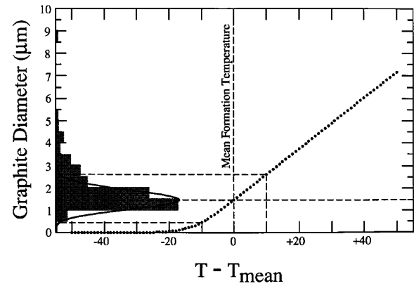
FIG. 15.—Example of the variation of graphite diameter (dotted curve) at the end of condensation as a function of seed appearance temperature, assuming a peak in seed formation at T = T_{\text{mean}} . The solid curve is the model size distribution given by eq. (9), superposed on the actual size distribution of onion-type circumstellar graphites (from Fig. 1). In this example, \sim 99\% of the seeds form within \pm 10 K of the mean appearance temperature. Assumed parameters were t_0 = 5 \times 10^6 s, n_g = 0.03 \text{ cm}^{-3} , and P = 10 \text{ dynes cm}^{-2} , with T_{\text{mean}} taken to be 50 K below the equilibrium condensation temperature at this pressure (cf. Table 2).
