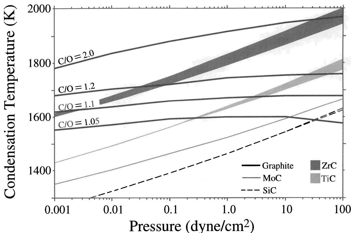
FIG. 10.—Equilibrium condensation temperatures for various carbides and graphites as a function of total pressure and C/O ratio (from 1.05 to 2). Solar abundances were used for all elements except carbon. Condensation temperatures for ZrC, TiC, and SiC vary slightly with C/O and are displayed as envelopes. For these compounds, the lower boundary of the envelope is for C/O = 1.05 , and the upper boundary is for C/O \geq 2.0 . For MoC, the condensation temperature does not vary with C/O in the displayed pressure range. The condensation temperature of \text{Mo}_2\text{C} (not shown) is only a few degrees higher than for MoC at any given pressure. The data are taken from Lodders & Fegley (1995).
