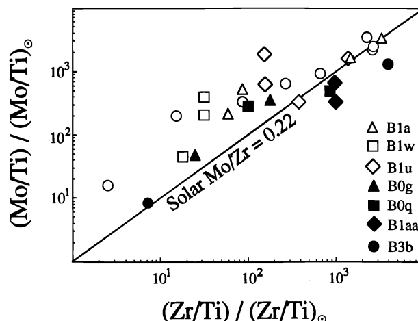
FIG. 9.—Comparison of Mo/Ti and Zr/Ti ratios (normalized to solar abundances) in carbide crystals within circumstellar graphite spherules that have measurable abundances of all three elements. Error bars have been suppressed for clarity (cf. Fig. 11 and Table 1). Only spherules having more than one crystal are listed in the legend; if only one crystal was measurable within a spherule, its composition is shown as an open circle. Solar composition plots in the lower left-hand corner, and the diagonal line is the locus of solar Mo/Zr ratios. The variations in elemental composition among crystals from individual spherules, and the substantial enrichments of Mo and Zr relative to Ti, point to chemical fractionation accompanying condensation of these crystals.
