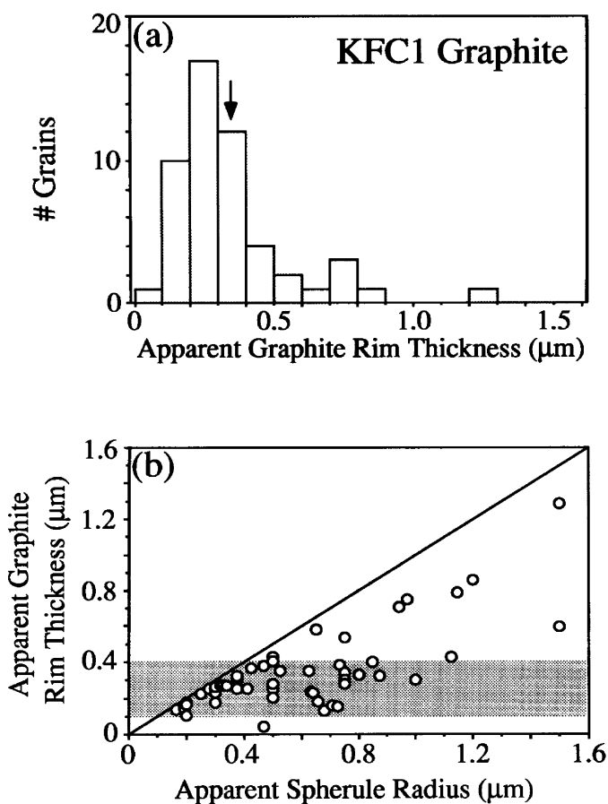
FIG. 6.—(a) Histogram of apparent graphitic outer shell (rim) thicknesses measured in ultrathin sections of circumstellar graphite spherules. The arrow denotes the mean thickness. (b) Apparent rim thickness vs. apparent graphite spherule radius. All data plot below the diagonal line, because the rim thickness cannot exceed the particle radius. Seventy-five percent of the spherules have rim thicknesses from 0.1 to 0.4 \mu\text{m} (shaded area), and there is no apparent correlation of rim thickness with grain size for spherules with rim thicknesses in this range.
