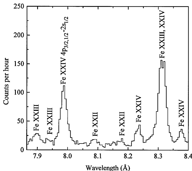
FIG. 2.—Fe xxiv 4 \rightarrow 2 spectrum at an electron beam energy of 4500 eV recorded for 155 minutes. The spectrum was collected using a thallium hydrogen phthalate crystal in first order.
