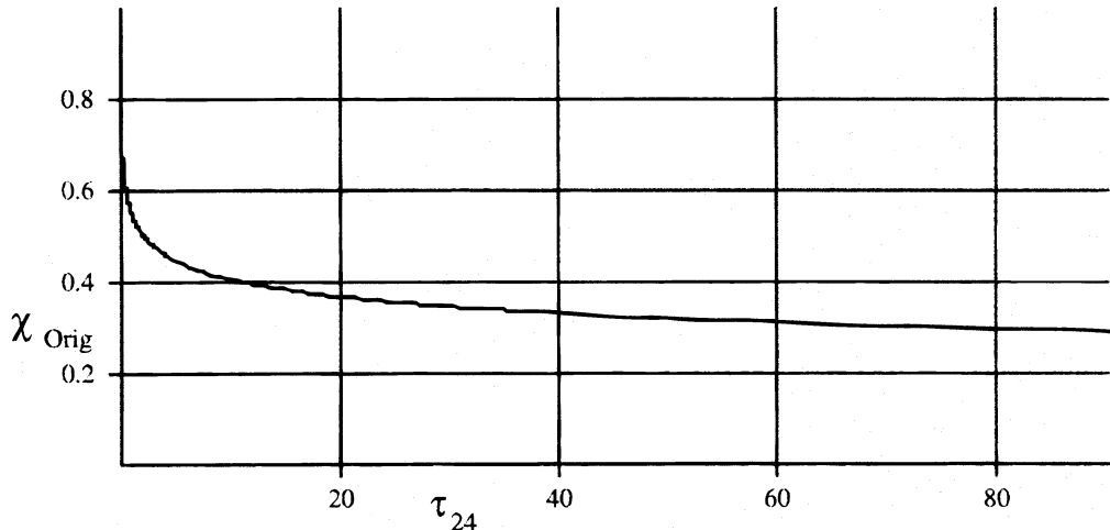
FIG. 3.—Starting \chi_{He} for no-recombination conditions vs. \tau_{24} . This is the recombination-equilibrium ionization where the Compton cooling ceases to dominate the heating. The steep slope near \tau_{24} = 0 reflects the fact that the heating approaches zero as \chi_{He} goes to one, so there needs to be a high photon production rate to compensate.
