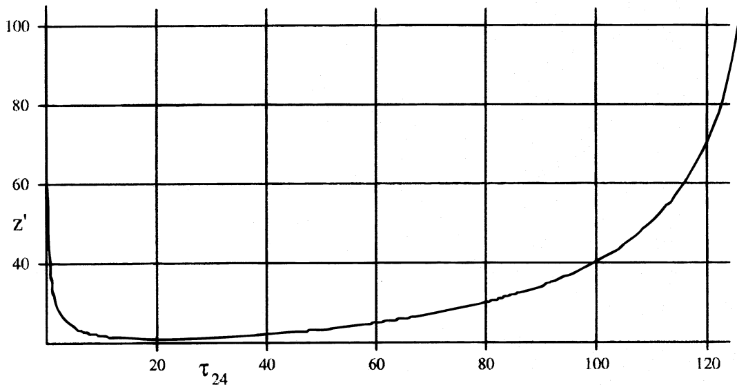
FIG. 1.—Minimum z' = z + 1 vs. \tau_{24} = \tau_\gamma/10^{24} . For small \tau_{24} (large photon production rate), the minimum redshift is large because the large equilibrium ionization leads to a large mean free path. For large \tau_{24} , the minimum redshift is large because the low ionization leads to low instability growth.
