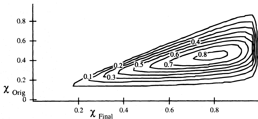
FIG. 4.—Logarithm of the total growth factor vs. the initial and final ionization for no-recombination growth. Since ionization increases with time, we clearly need the final ionization to be larger than the initial ionization, with larger values of their difference giving more time for growth. However, very small values for the original ionization correspond to low photon production rates, which give small overall growth. Large values for the final ionization correspond to large spatial scales, where the growth is also reduced.
