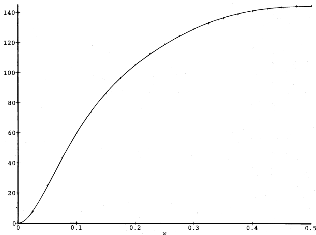
FIG. 5.—He 2^1S two-photon decay rate vs. energy ( x = \nu/E_4 ). The fitting formula is A(x) = -0.98p(2, x) + 2.83p(3, x) - 4.26p(4, x) + 2.15p(5, x) , where p(j, x) = 300\{(2x - 1)^{2j} - 1 - j[(2x - 1)^2 - 1]\} (this form is chosen so that each term is symmetric around x = 0.5 and is zero and has zero slope at x = 0 and x = 1 ). The rms error of the fit is 0.34.
