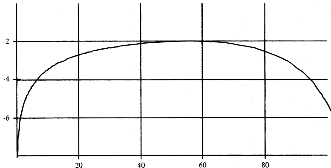
FIG. 2.— \mathcal{L}_n/\mathcal{P}_n vs. \tau_{24} . The curve follows the inverse of the minimum z' curve (since Compton cooling is much more effective at large z ), with a shift toward larger \tau_{24} (where the ionization and thus the cooling is less).
