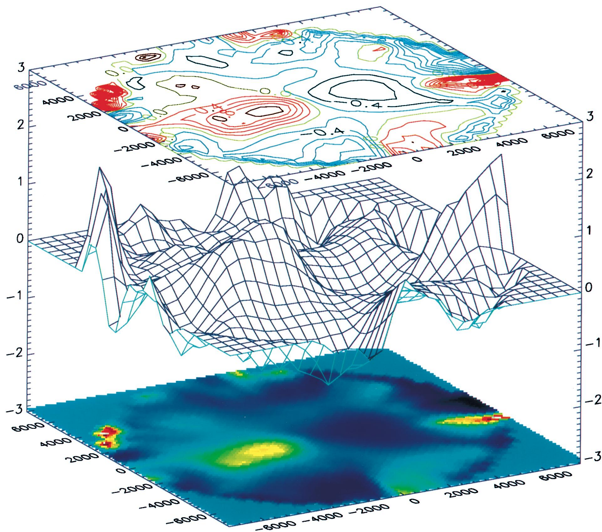
FIG. 1.—Density field along the supergalactic plane reconstructed from the SFI sample. We show density contours in intervals of \delta = 0.2 , surface density maps with the height proportional to \delta and density contrast maps. Bright yellow represents overdensities and dark blue underdense regions, respectively. See text or Fig. 2 for the identification of the structures.
