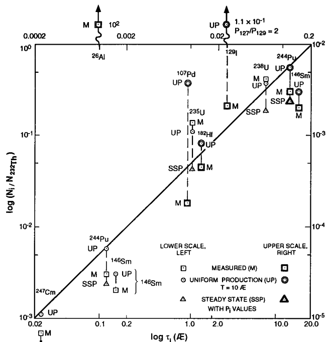
FIG. 1.—Graph of \log(N_i/N_{232\text{Th}}) vs. \log \bar{\tau}_i . Solid line corresponds to steady state with P_i^{\text{AC}} = \text{const.} For standard production rates, P_i^{\text{AC}} ; \triangle for SSP; \odot for uniform production over 10^{10} yr; and \square for observed values.
