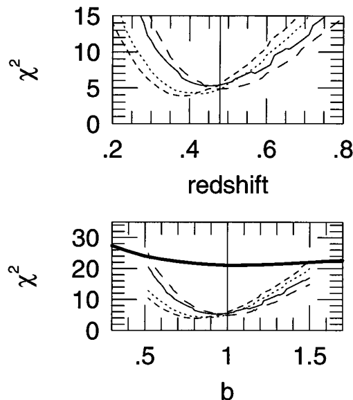
FIG. 1.— \chi^2 distributions for different values of the fitting parameters. For each calculation, the other parameter has been set to the canonical values, i.e., z = 0.479 and b = 1 . The curves are for SN 1990N (solid lines), SN 1991T (dotted lines), SN 1992bc (short-dashed lines), and the average template (long-dashed lines). The heavy line is the result from the LCS fitting.
