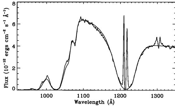
FIG. 4.—Ly \beta and Ly \alpha region of the background-subtracted HUT spectrum compared with a theoretical model ( smooth curve ) with the new Ly \alpha broadening including the quasi-molecular satellites and T_{\text{eff}} = 20,000 K, \log g = 7.90 .
