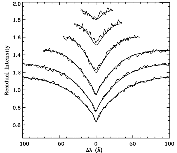
FIG. 2.—Balmer line profiles of Wolf 1346 and the best-fitting model with T_{\text{eff}} = 19504 \text{ K} , \log g = 7.96 . Lines shown are H \beta through H9.
