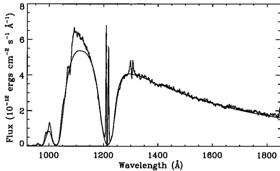
FIG. 1.—Background-subtracted HUT spectrum of Wolf 1346, compared with a theoretical spectrum using standard Ly \beta Stark broadening. The Ly \alpha and O II airglow lines at 1216 and 1304 Å could not be subtracted cleanly due to the decline in sensitivity in those lines through the mission.
