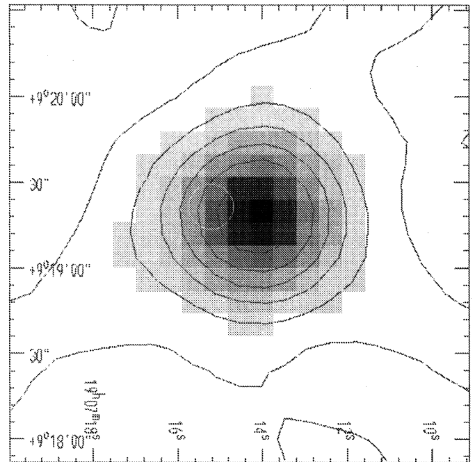
FIG. 3.—Enlargement of the area around source 1. The two infrared sources in Vrba et al. (1996) are located at the center of the circle.
