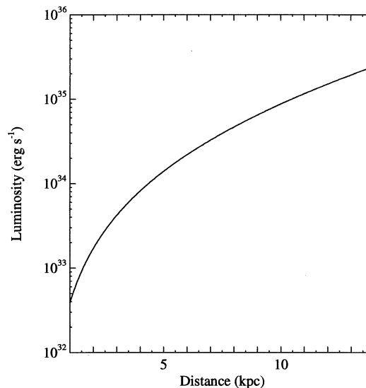
FIG. 2.—Source luminosity as a function of assumed distance. The total column density in this direction, 10^{22} cm -2 (determined using the HEASARC on-line service) along a line of sight of 14 kpc, has been scaled linearly to the distance.
