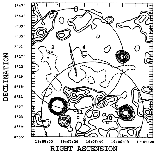
FIG. 1.— ROSAT observations and 327 MHz radio contours. X-ray sources are shown as squares whose sizes are equal to the detection cell size (see Table 1). Sources 5 and 6 encompass sources 2 and 3; in the interest of clarity, they are not shown. Sources 7, 9, and 12 may be associated with features in G42.8+0.6. The two circles represent the ROSAT HRI fields of view for the two pointings. The diamond-shaped network synthesis error box of SGR 1900+14 is also shown.
