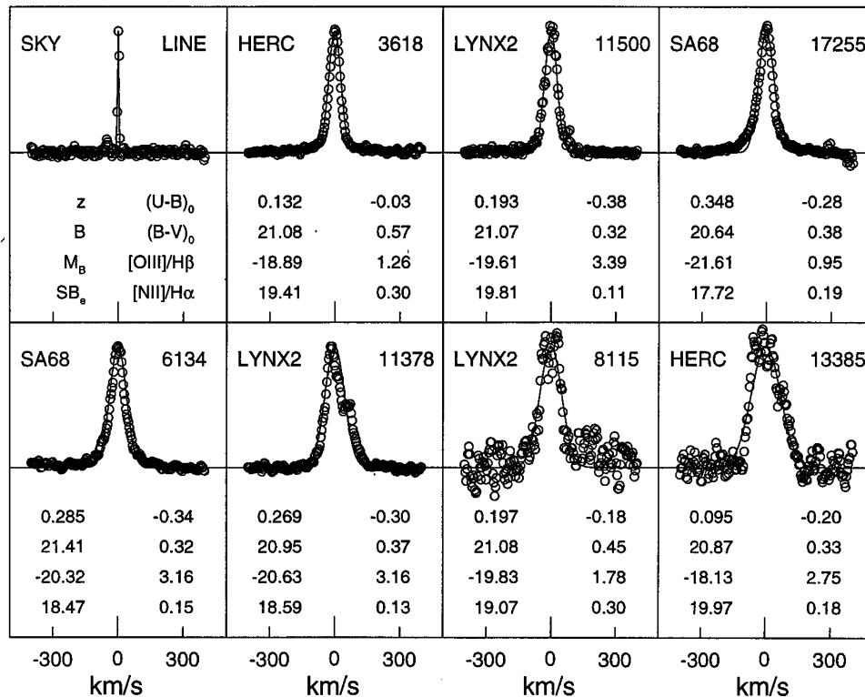
FIG. 1.—Panel of new [O III] \lambda 5007 emission-line profiles in \text{km s}^{-1} for five CNELGs. For completeness, we also show the emission-line profiles of Her 13385 and Her 3618 (Koo et al. 1995). In the upper left panel, a typical night sky line shows our instrumental resolution of \sigma = 3.4 \text{ km s}^{-1} . Each panel is labeled at the top with the ID name (field and number) and includes the redshift ( z ), apparent blue B , magnitude, rest-frame B absolute magnitude ( M_B ), rest-frame B surface brightness in \text{mag arcsec}^{-2} ( SB_e ), rest-frame U - B and B - V colors, and [O III] \lambda 5007/H\beta and [N II] \lambda 6583/H\alpha line ratios, in positions as shown in the upper left panel. Solid lines show the best Gaussian curve that fits the average of profiles from all emission lines. Note the presence of a second component in Lyn 2-11378 and the extended wings in SA 68-17255.
