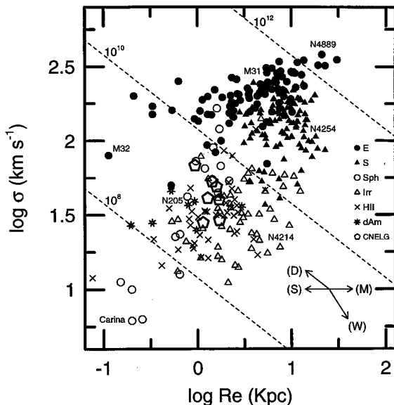
FIG. 2.—The half-light radius ( R_e ) vs. velocity width ( \sigma ) diagram for various galaxy types: open pentagons , CNELGs (this paper); filled circles , E/S0 galaxies (Bender et al. 1992); filled triangles , spirals (de Vaucouleurs et al. 1991); open triangles , irregulars (de Vaucouleurs et al. 1991); open circles , spheroidals (Bender et al. 1992); crosses , H II galaxies (Telles 1995) and stars , dwarf amorphous galaxies (Marlowe et al. 1994). For convenience, a few galaxies representative of today’s evolved stellar systems have been identified. The arrows represent the direction in which R_e and \sigma change due to different physical processes as explained in the text: (D) dissipation; (M) mergers; (S) tidal stripping; (W) galactic winds. The dashed lines correspond to constant-mass lines of 10^8 , 10^{10} , and 10^{12} solar masses, respectively. Along these lines, mass surface-density decreases uniformly from the upper left to the bottom right part of the diagram.
